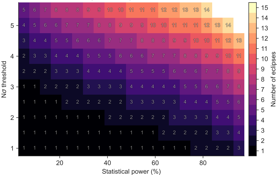
Checkpoint 2 Eclipses for TOI-244 b
