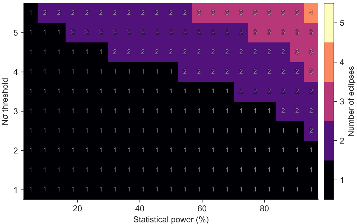
Checkpoint 1 Eclipses for LTT 1445 A c
