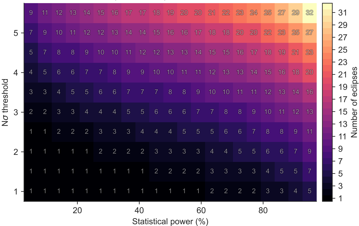
Checkpoint 2 Eclipses for LHS 1140 b
