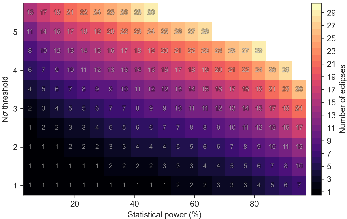
Checkpoint 2 Eclipses for TOI-406 c
