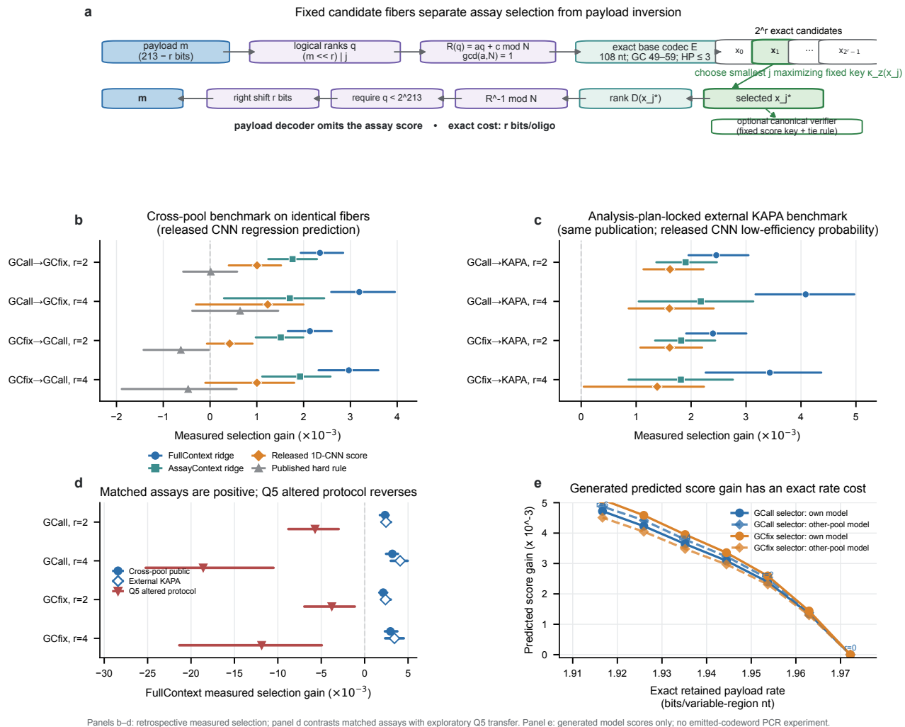
Fig. 2: Exact reversible choice coding and retrospective assay-guided selection. (a) Full-language modulo- N choice coding and scorer-independent payload inversion. (b,c) Retrospective measured selected-minus-fiber-mean PCR-efficiency gains on fixed GCall/GCfix and external-KAPA fibers; released CNN endpoints differ. Whiskers are marginal 95% BCa intervals from 2,000 target-fiber resamples. (d) Grouped-source plus target-fiber two-stage 95% intervals show positive matched-assay gains and negative secondary exploratory Q5 gains on a common zero axis. All intervals condition on published sequence-level outcomes and exclude technical-replicate, batch, normalization and assay-measurement uncertainty. (e) Predicted generated-codeword score-rate trade-off per 108-nt variable region. Generated candidates were computationally verified but not synthesized or assayed. Complete definitions and intervals are in Supplementary Information.
