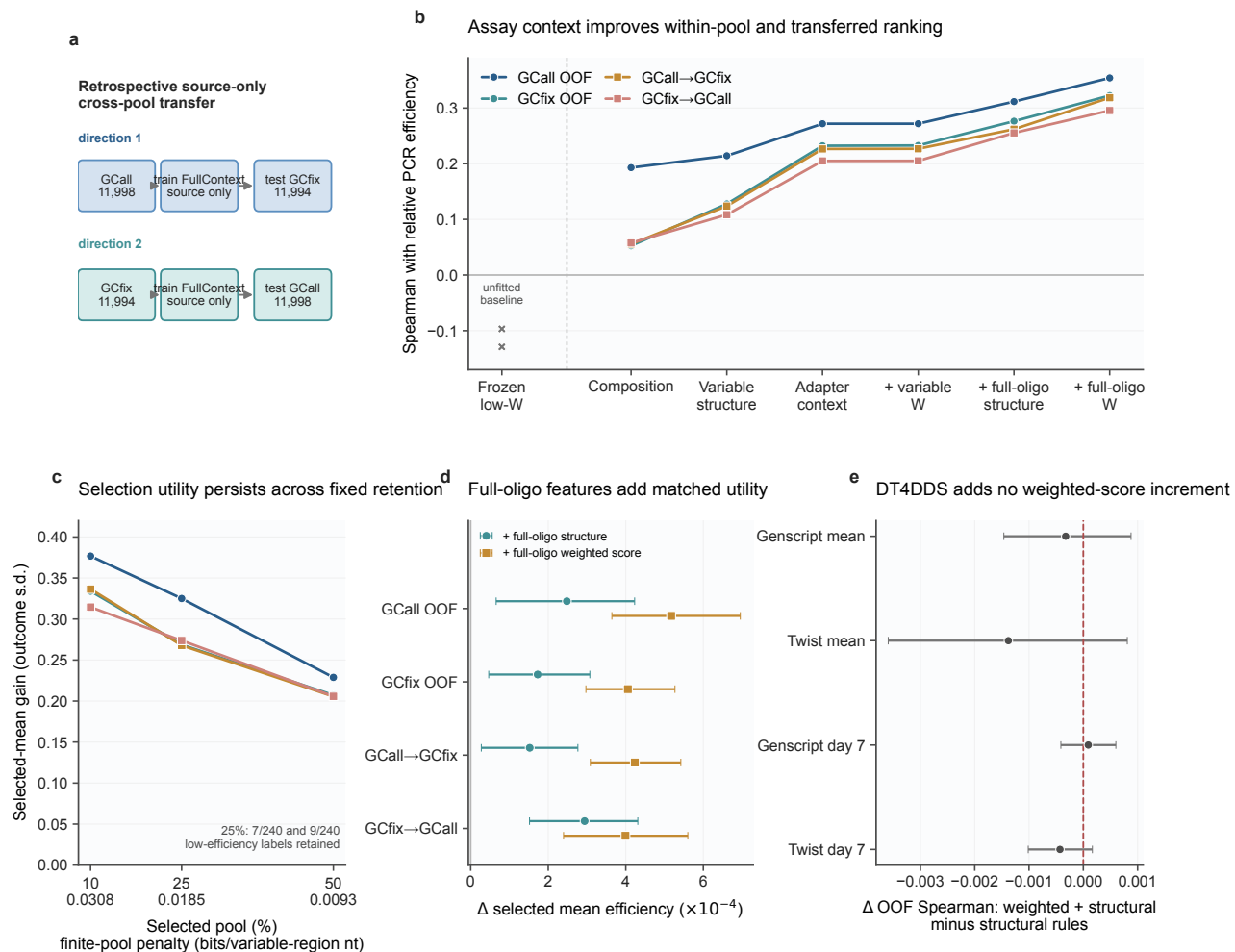
Fig. 1: Retrospective assay-context modelling in public measured libraries. (a) Outcome-excluded source-only transfer between GCall ( n = 11,998 ) and GCfix ( n = 11,994 ), with exhaustive fixed-length Hamming audit. (b) Spearman correlation with measured PCR efficiency; F0 is unfitted and P0–P5 are nested ridge models. OOF denotes five repeated nested five-fold predictions. (c) Measured retained-set gains. (d) Paired 25%-retention increments from complete-oligonucleotide features; whiskers are percentile 95% intervals from 2,000 sequence bootstraps without model refitting. Intervals condition on published sequence-level outcomes and exclude assay-measurement uncertainty. (e) Null change in measured DT4DDS abundance ranking. Public sequences were not codec outputs; no panel is prospective emitted-sequence PCR.
