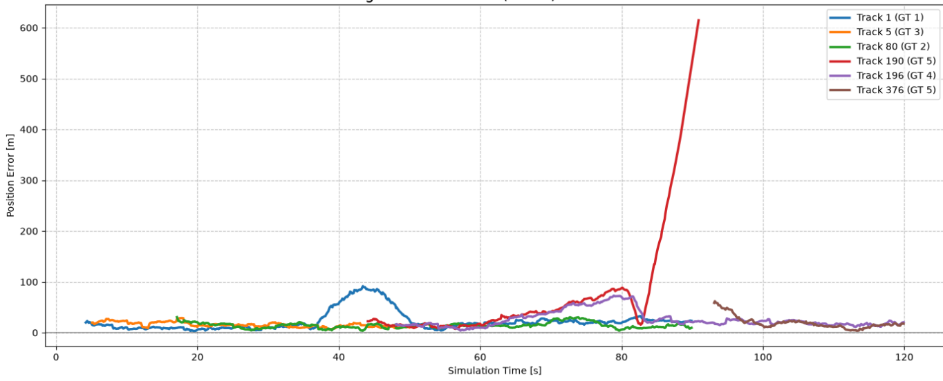
Fig 7: Position Error (RMSE) over Time
