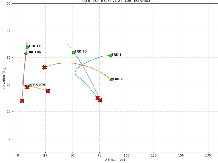
Fig 6: EKF Tracks vs GT (Left: EO View)
