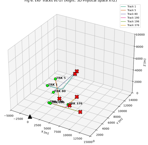
Fig 6: EKF Tracks vs GT (Right: 3D Physical Space XYZ)
