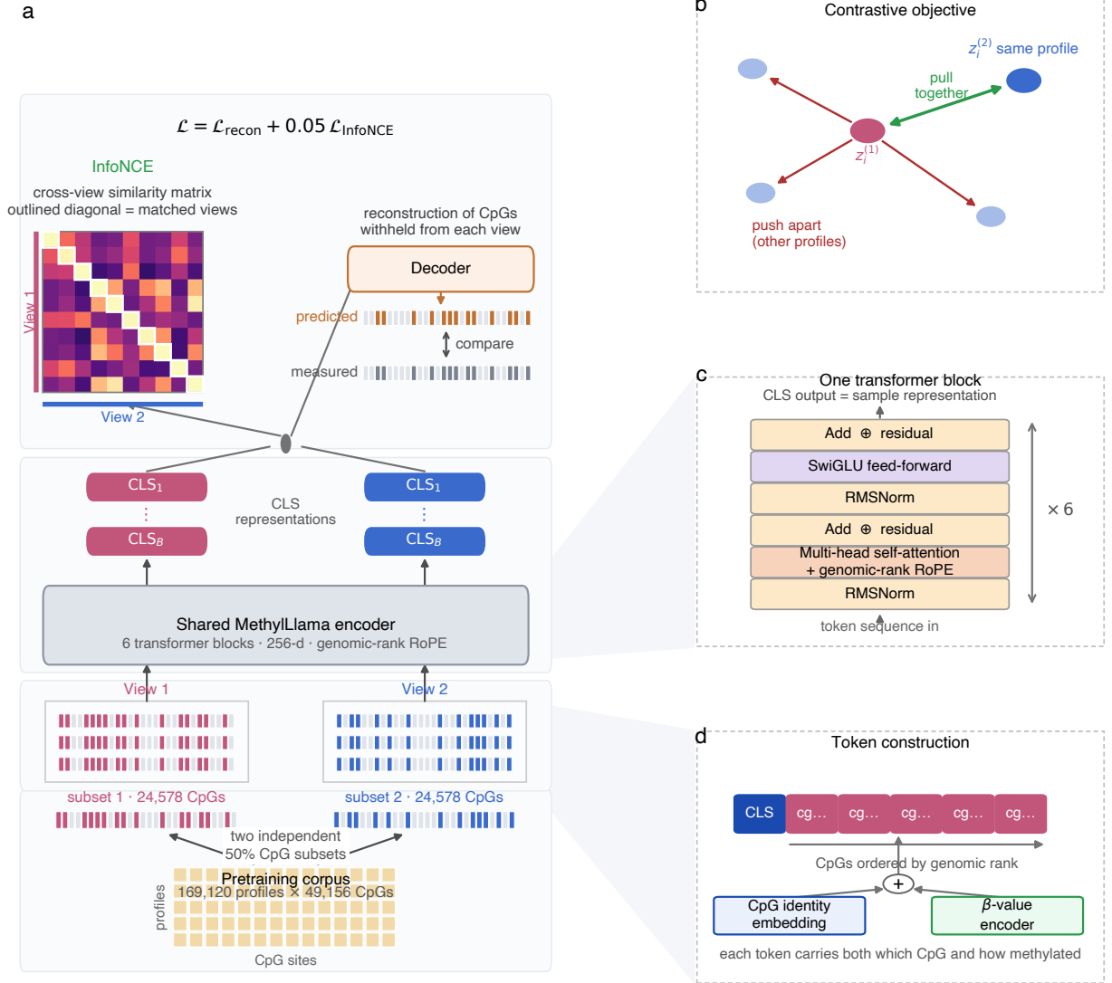
Figure 1: Study design and self-supervised pretraining of Methylllama. a , Study design. The unlabelled pretraining corpus is distinguished from the labelled AltuMAGE evaluation collection, and the two downstream analysis populations are shown separately: the 10,988-profile partition used for frozen-representation probes and the filtered, deduplicated 2,149-sample test set used for supervised comparisons. Phenotype annotations were not used as supervision during pretraining. b , View construction. Two independent 50% subsets of the measured CpGs of one profile form the two views; for each view, the complement (hatched) provides the reconstruction target, so the objective is scored only at measured CpGs absent from that view. c , The WCED objective. A shared encoder maps each view to a CLS representation; a decoder predicts the withheld CpGs from that representation alone, and a symmetric InfoNCE term aligns the two projected CLS embeddings. d , Token encoding. Each CpG token sums a learned site-identity embedding and a continuous \beta -value encoding, with a CLS token prepended to every partial profile.
