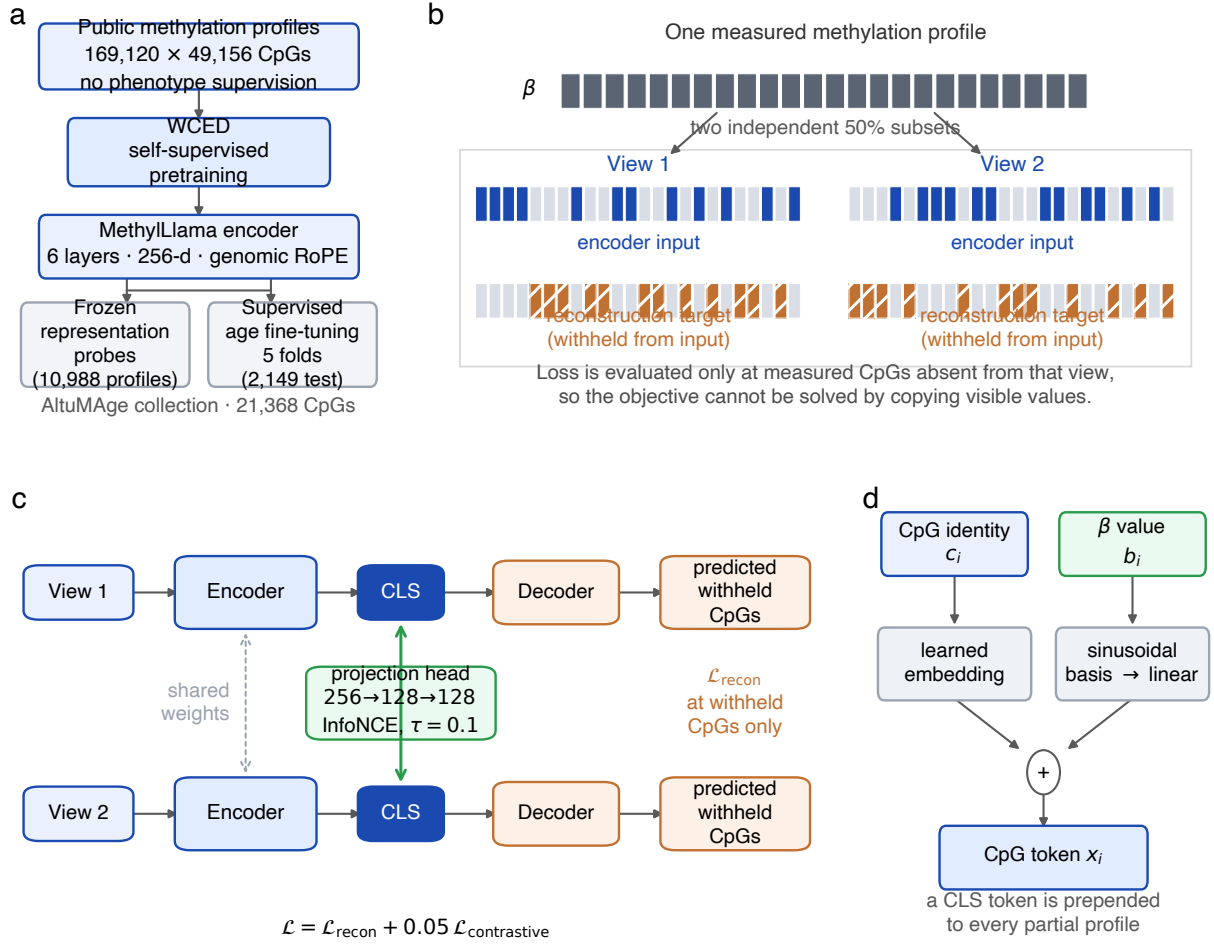
Figure 1: Study design and self-supervised pretraining of MethyLLama. a , Study design. The unlabelled pretraining corpus is distinguished from the labelled AltumAge evaluation collection, and the two downstream analysis populations are shown separately: the 10,988-profile partition used for frozen-representation probes and the filtered, deduplicated 2,149-sample test set used for supervised comparisons. Phenotype annotations were not used as supervision during pretraining. b , View construction. Two independent 50% subsets of the measured CpGs of one profile form the two views; for each view, the complement (hatched) provides the reconstruction target, so the objective is scored only at measured CpGs absent from that view. c , The WCED objective. A shared encoder maps each view to a CLS representation; a decoder predicts the withheld CpGs from that representation alone, and a symmetric InfoNCE term aligns the two projected CLS embeddings. d , Token encoding. Each CpG token sums a learned site-identity embedding and a continuous \beta -value encoding, with a CLS token prepended to every partial profile.
