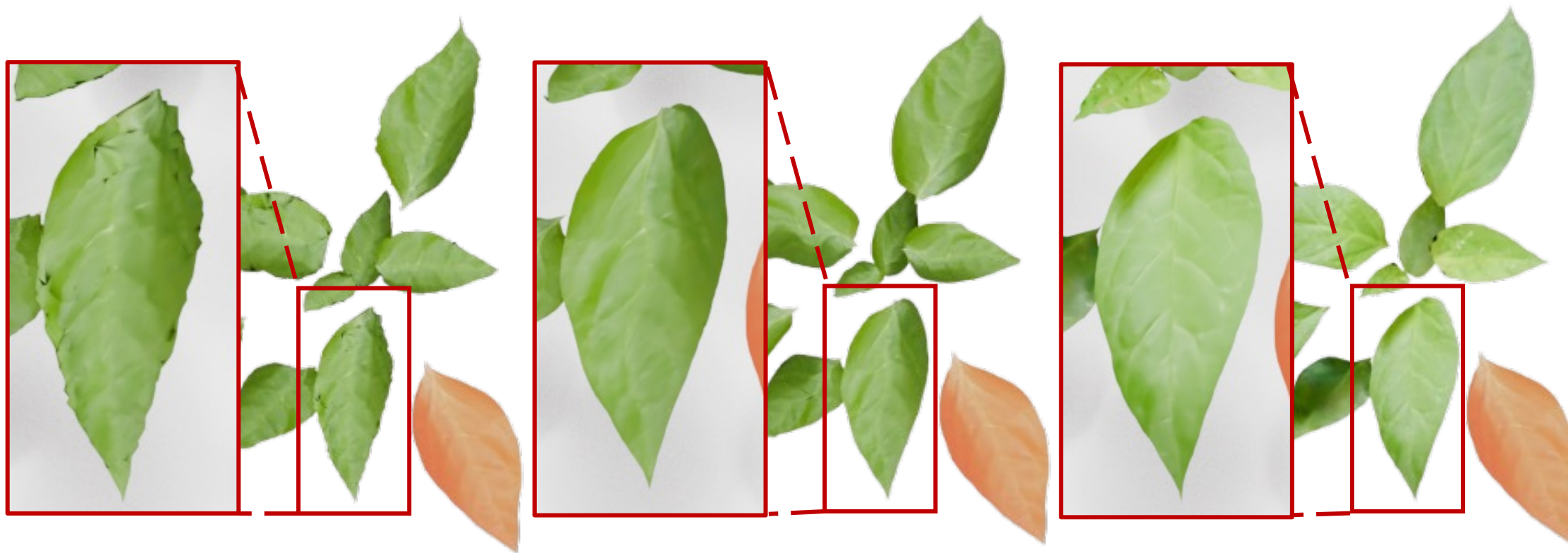
Non-Rigid ICP
