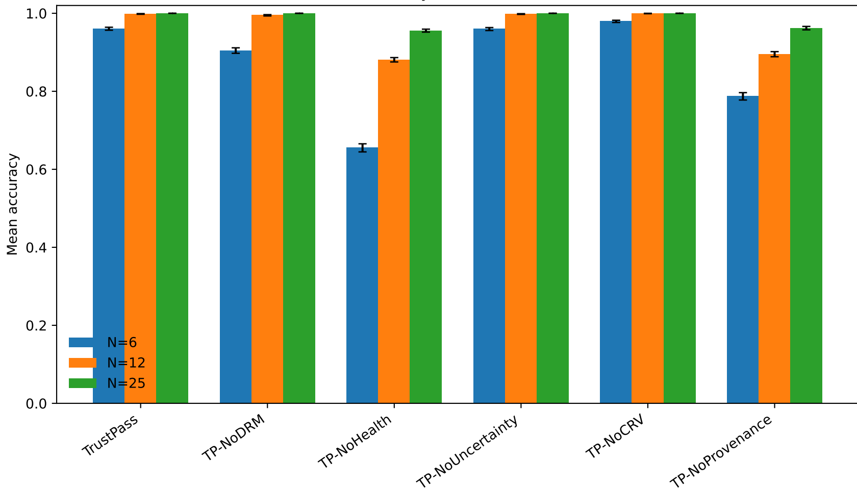
TrustPass ablation study with 95% confidence intervals
