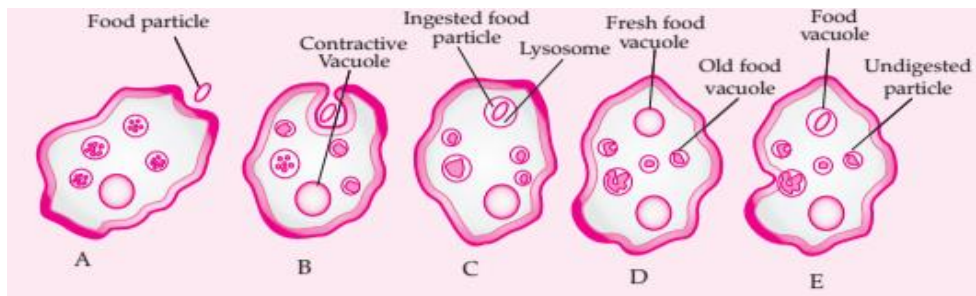
Holozoic nutrition in Amoeba
