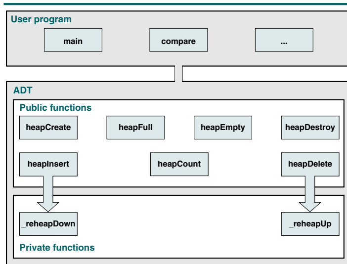
FIGURE 9-12 Heap ADT Design
