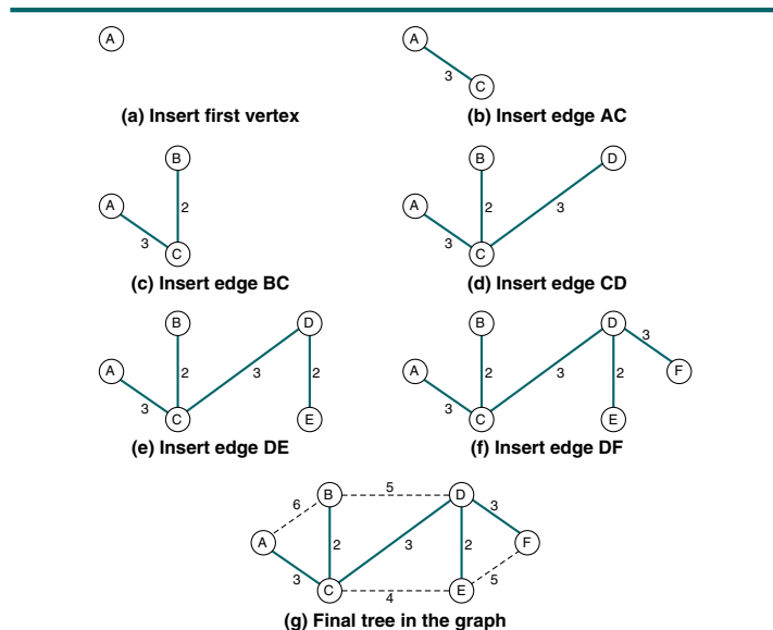
FIGURE 11-21 Develop a Minimum Spanning Tree
