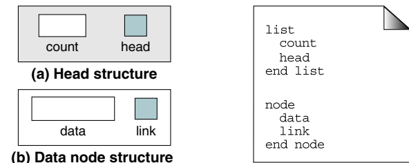
FIGURE 5-5 Head Node and Data Node
