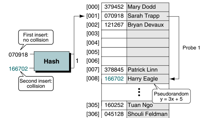
FIGURE 13-16 Pseudorandom Collision Resolution
