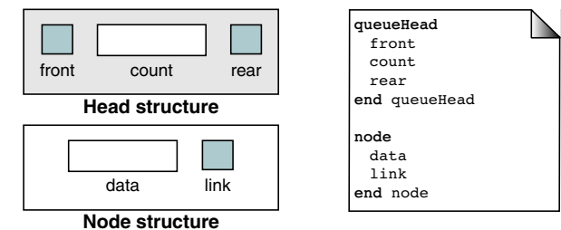
FIGURE 4-8 Queue Data Structure
