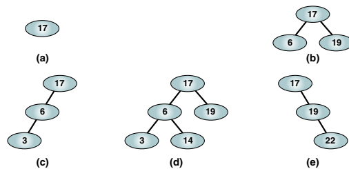
FIGURE 7-2 Valid Binary Search Trees
