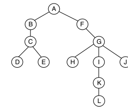
FIGURE 6-25 Tree for Exercises 2, 3, 4, 5, 6, and 7
