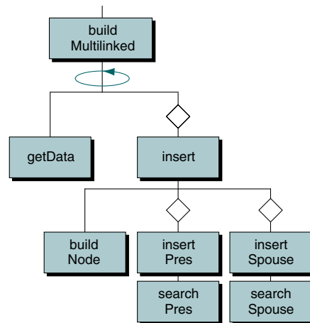
FIGURE 5-24 Multilinked List Add Node
