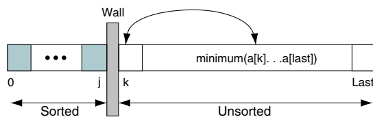
FIGURE 12-3 Selection Sort Concept
