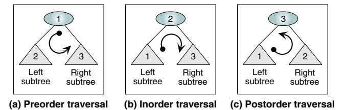
FIGURE 6-8 Binary Tree Traversals
