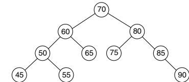
FIGURE 7-22 Figure for Exercises 13 and 14
