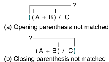
FIGURE 3-14 Unmatched Parentheses Examples
