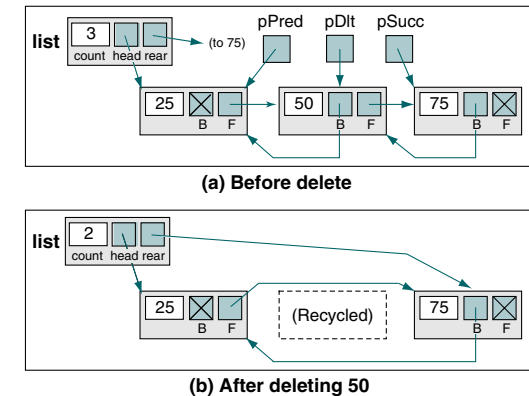
FIGURE 5-22 Doubly Linked List Delete
