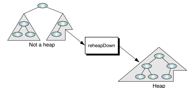
FIGURE 9-6 Reheap Down Operation
