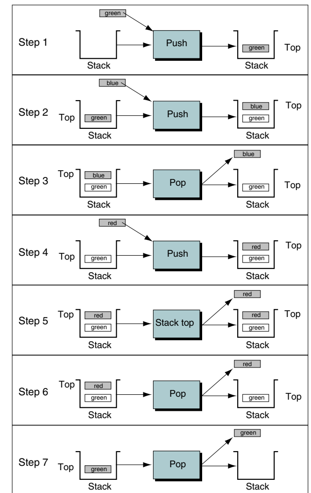
FIGURE 3-5 Stack Example
