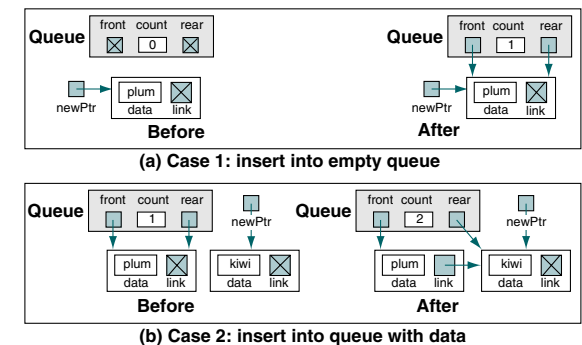
FIGURE 4-10 Enqueue Example
