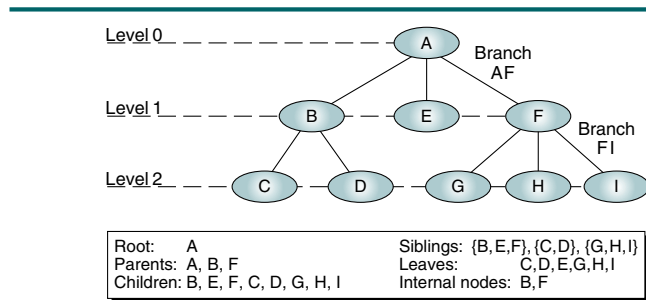
FIGURE 6-2 Tree Nomenclature
