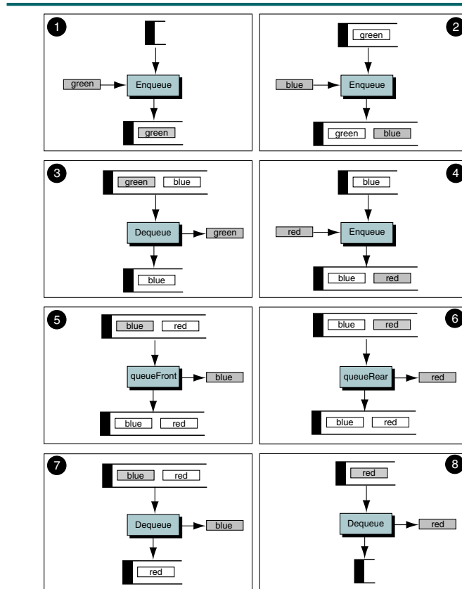
FIGURE 4-6 Queue Example
