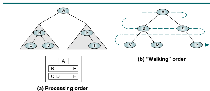
FIGURE 6-14 Breadth-first Traversal
