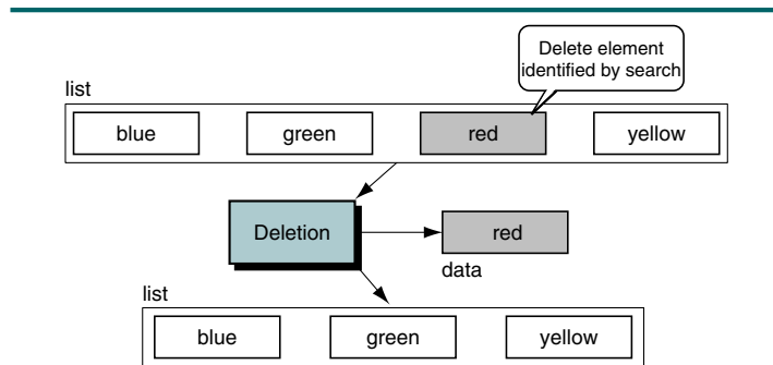
FIGURE 5-2 Deletion
