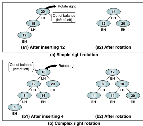
FIGURE 8-4 Left of Left—Single Rotation Right
