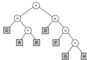
FIGURE 6-27 Expression Tree for Exercise 26
