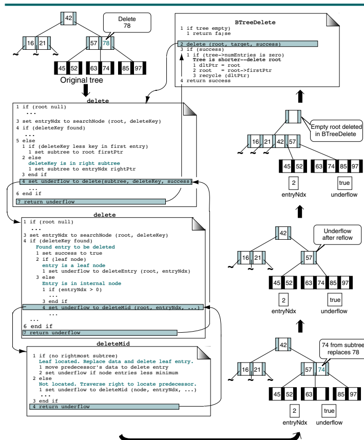
FIGURE 10-11 B-tree Deletions
