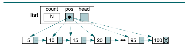
FIGURE 5-14 List Traversal
