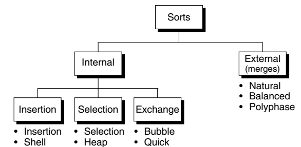
FIGURE 12-1 Sort Classifications
