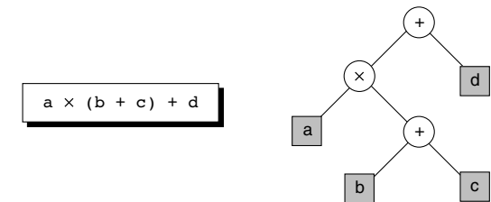
FIGURE 6-15 Infix Expression and Its Expression Tree
