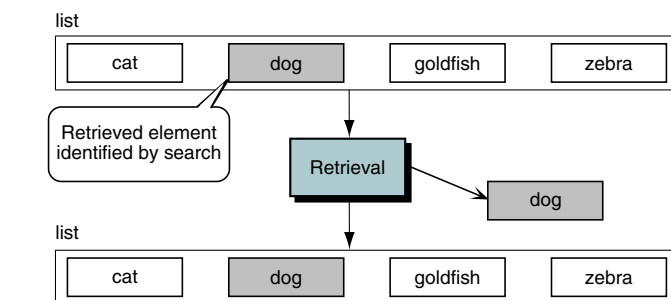
FIGURE 5-3 Retrieval
