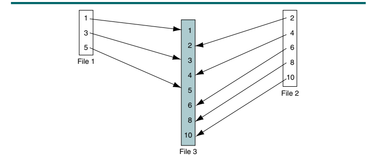
FIGURE 12-17 Simple Merge
