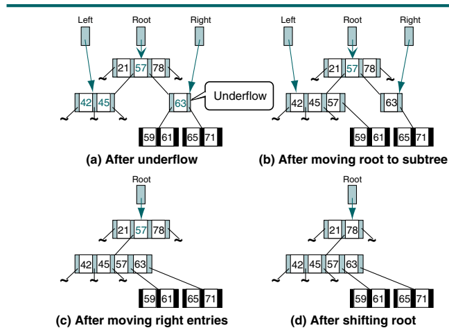
FIGURE 10-13 B-tree Combine
