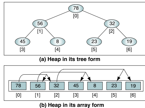
FIGURE 12-5 Heap Representations
