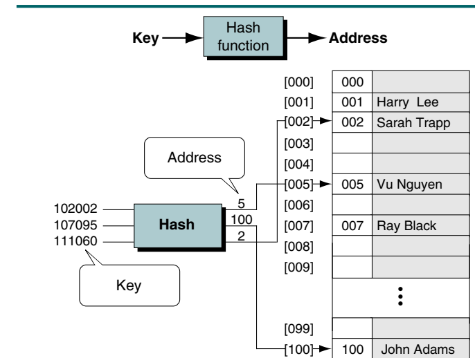
FIGURE 13-6 Hash Concept
