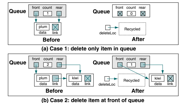
FIGURE 4-11 Dequeue Examples
