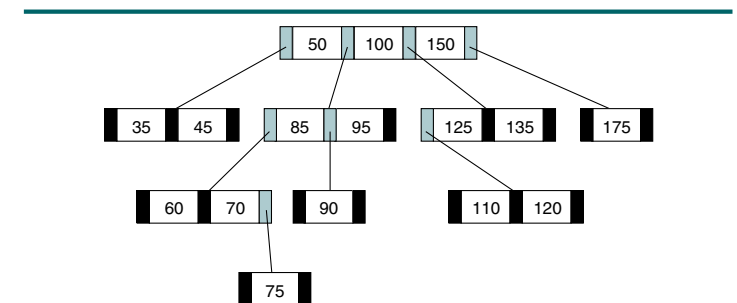
FIGURE 10-2 Four-way Tree
