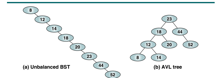
FIGURE 8-1 Two Binary Trees
