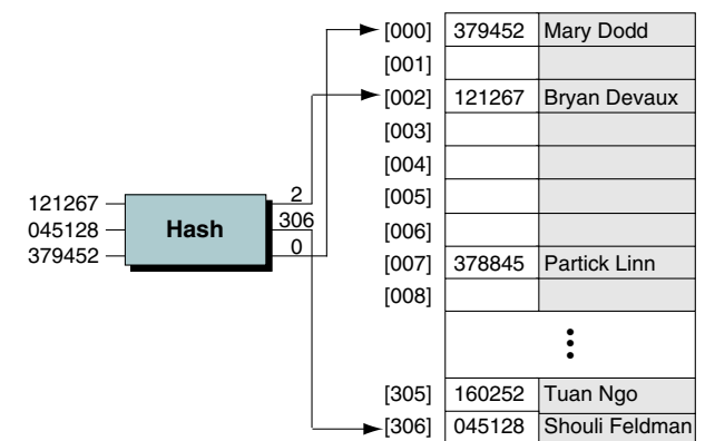
FIGURE 13-10 Modulo-division Hashing
