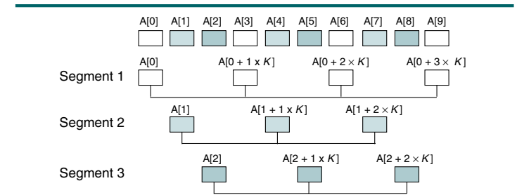
FIGURE 12-9 Segmented Array
