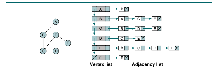
FIGURE 11-14 Adjacency List
