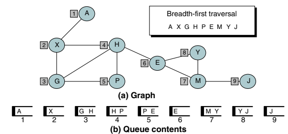
FIGURE 11-12 Breadth-first Traversal of a Graph
