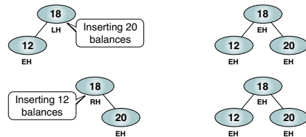
FIGURE 8-8 Automatic AVL Tree Balancing
