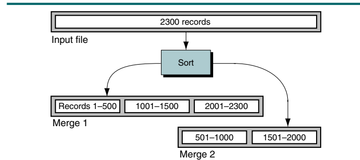
FIGURE 12-19 Sort Phase in an External Sort
