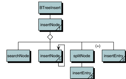
FIGURE 10-6 B-tree Insert Design
