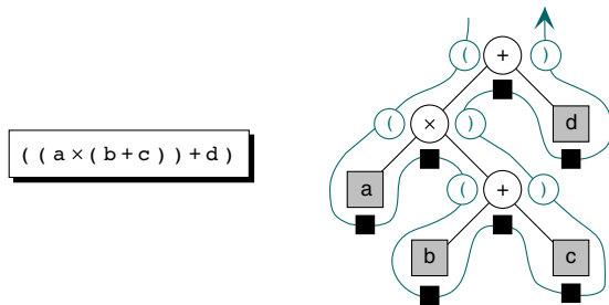
FIGURE 6-16 Infix Traversal of an Expression Tree
