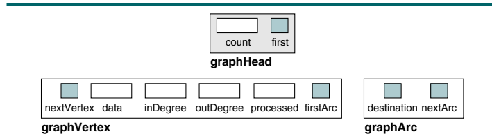
FIGURE 11-15 Graph Data Structure
