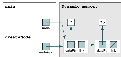
FIGURE 1-10 Structure for Two Linked Nodes
