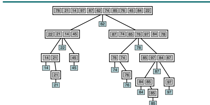
FIGURE 12-16 Quick Sort Operation
