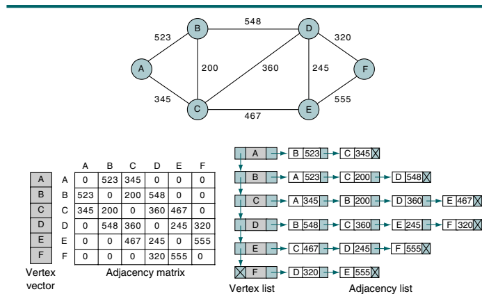
FIGURE 11-19 Storing Weights in Graph Structures
