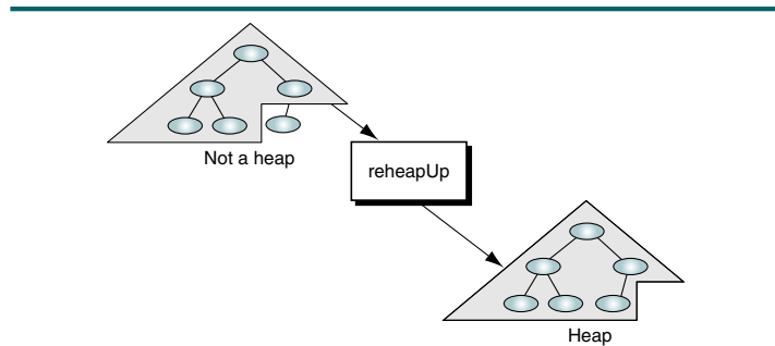
FIGURE 9-4 Reheap Up Operation
