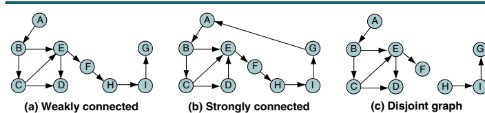
FIGURE 11-3 Connected and Disjoint Graphs
