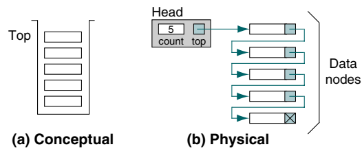
FIGURE 3-6 Conceptual and Physical Stack Implementations
