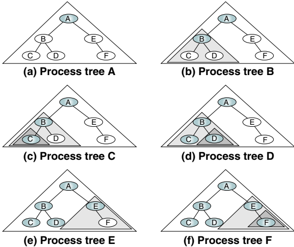
FIGURE 6-11 Algorithmic Traversal of Binary Tree
