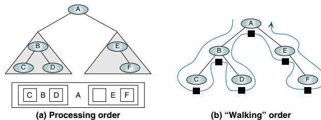
FIGURE 6-12 Inorder Traversal—C B D A E F
