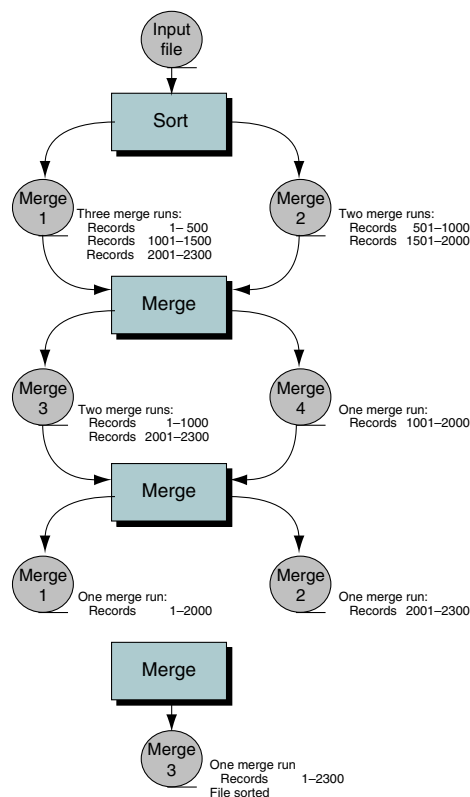
FIGURE 12-21 Balanced Two-way Merge Sort
