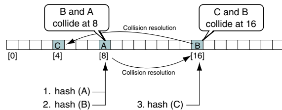
FIGURE 13-7 Collision Resolution Concept
