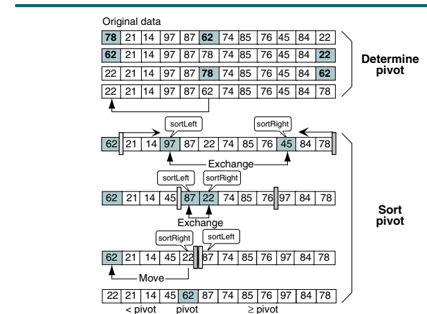
FIGURE 12-15 Quick Sort Pivot
