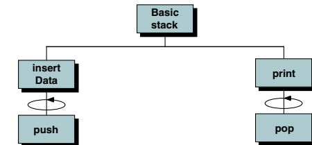
FIGURE 3-11 Design for Basic Stack Program
