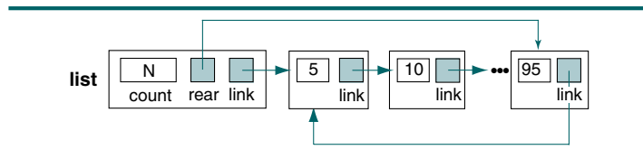
FIGURE 5-19 Circularly Linked List
