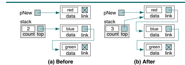
FIGURE 3-9 Push Stack Example
