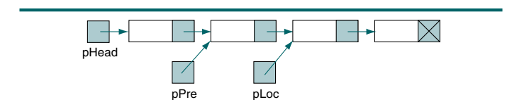
FIGURE 5-26 Linked List Implementation for Exercise 2
