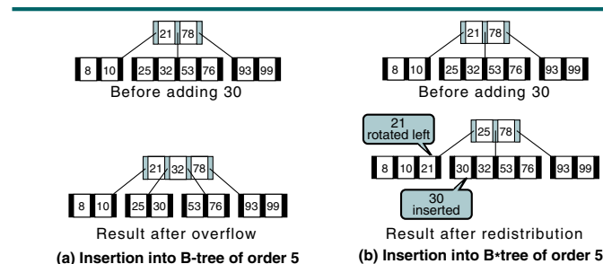
FIGURE 10-20 B*tree Insertion
