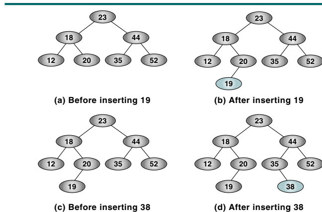
FIGURE 7-8 BST Insertion
