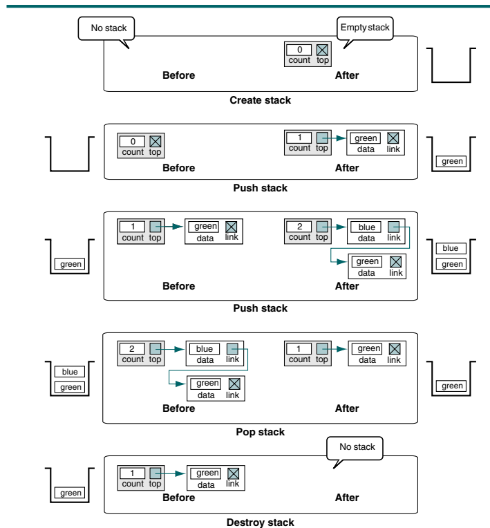
FIGURE 3-8 Stack Operations
