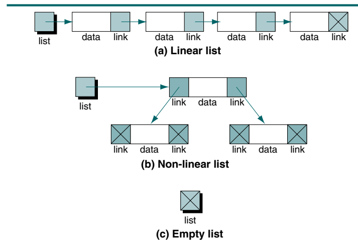
FIGURE 1-3 Linked Lists
