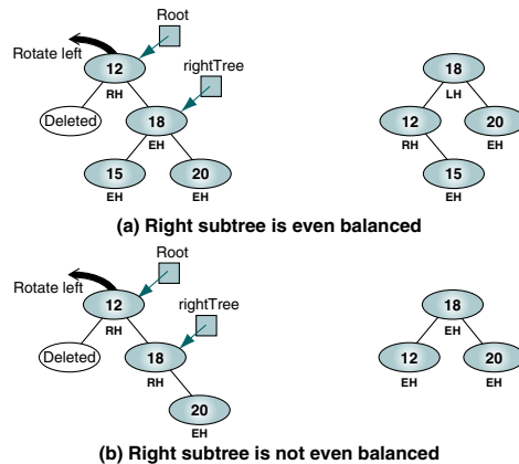
FIGURE 8-11 AVL Tree Delete Balancing
