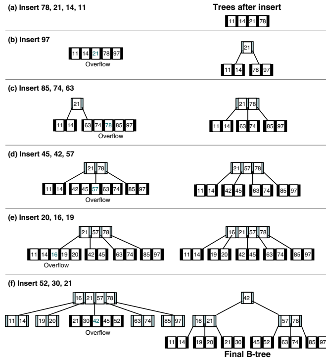
FIGURE 10-9 Building a B-tree of Order 5
