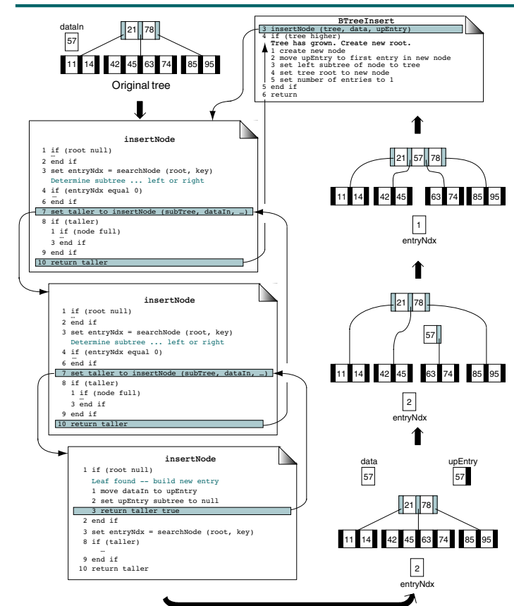
FIGURE 10-7 Build B-tree, First Overflow
