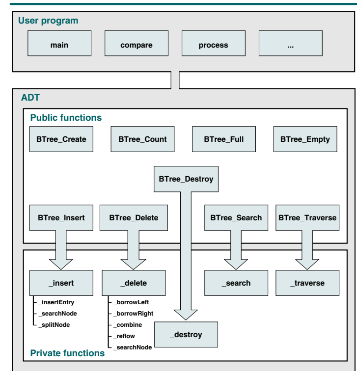
FIGURE 10-16 B-tree Function Family
