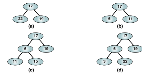
FIGURE 7-3 Invalid Binary Search Trees
