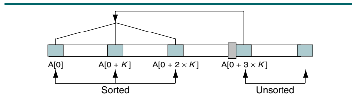
FIGURE 12-11 Ordered Segment in a Shell Sort
