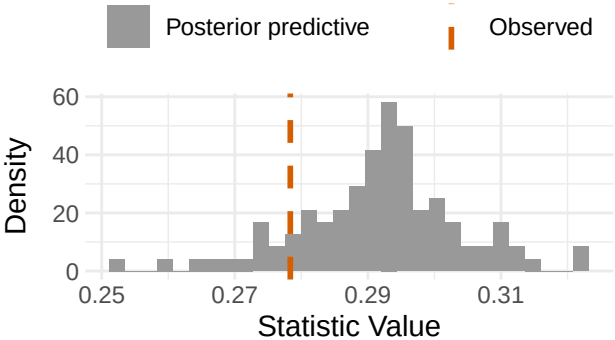
Triadic Dependence
