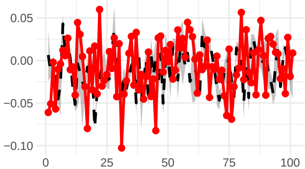
Triadic Dependence
