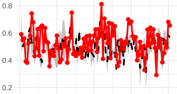
Transitivity
