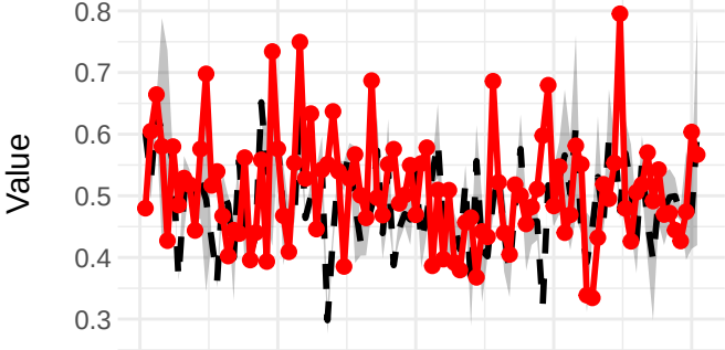
Triadic Dependence
