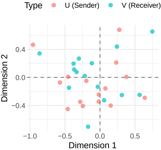
Multiplicative Effects
