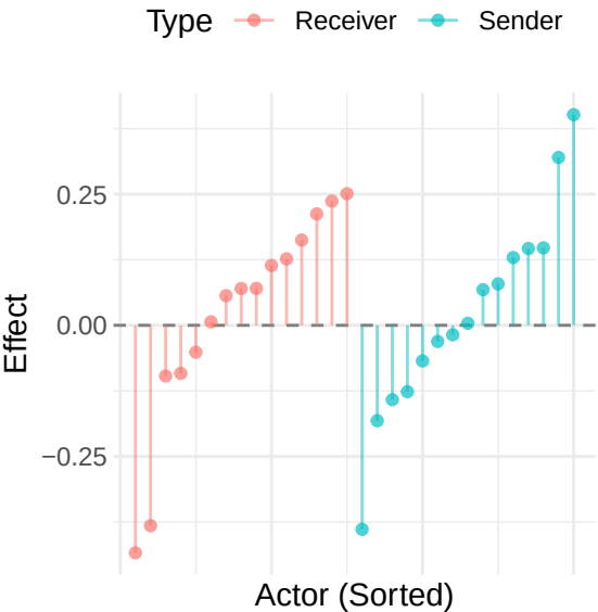
Multiplicative Effects
