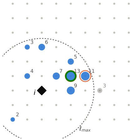
(a) R1: most visited, f_{v,i}(j) \geq c/2
