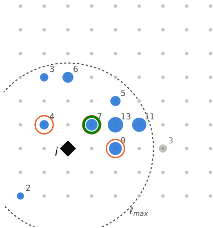
(b) R2: uniform at geodesic distance 2
