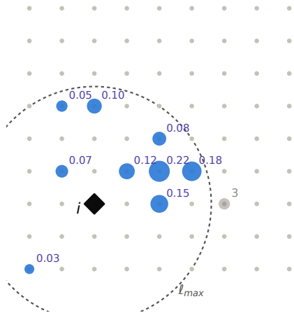
(c) R3: probability \propto f_{v,i}(j)
