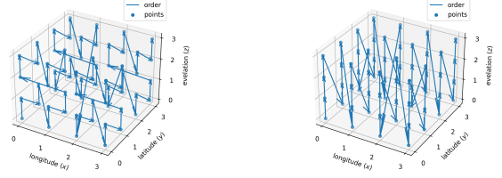
(a) 3D Z-Order Curve
