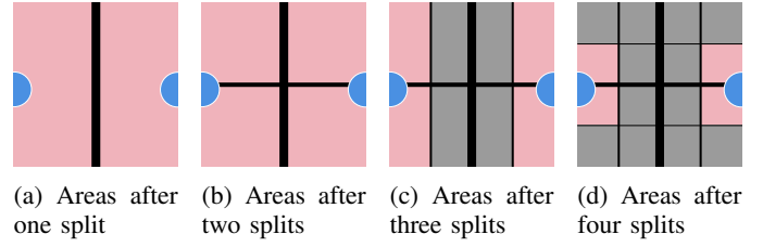
Fig. 4: The two-dimensional surface (longitude, latitude) after the first, second, third and fourth split. The blue circle shows a possible area to be claimed by a certificate or the desired query area of a client. The area colored in red is the minimum area that has to be retrieved using the given number of splits.
