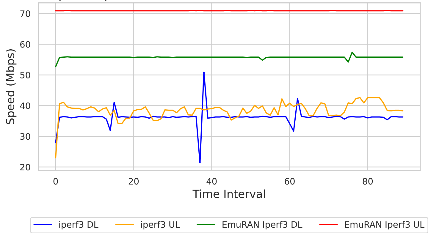
Iperf3 Speeds for EmuRAN vs vanilla srsRAN Emulation
