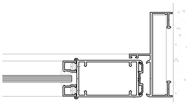
Corte 11"-11"
