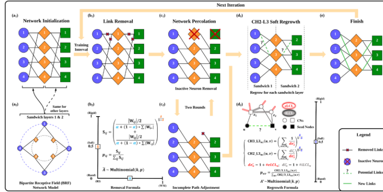
Figure 2: Illustration of the CHTs process. One training iteration follows the path of (a1) Network initialization \rightarrow (b1) Link removal \rightarrow (c1) Removal of inactive neurons caused by link removal \rightarrow (c2) Adjust and remove incomplete links caused by inactive neuron removal \rightarrow (d1) Link Regrowth \rightarrow (e) Finished state of the network after one iteration.
