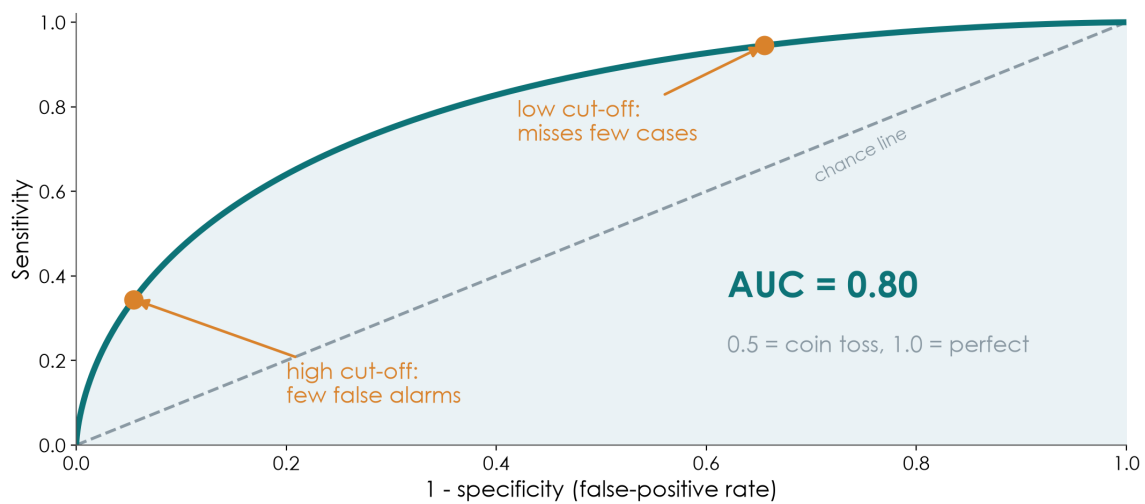
Figure 8.3: A receiver operating characteristic curve for a simulated test: each point is one cut-off, low cut-offs miss few cases but raise many false alarms, high cut-offs do the opposite, and the area under the curve is 0.80, compared with 0.5 for the chance line.
