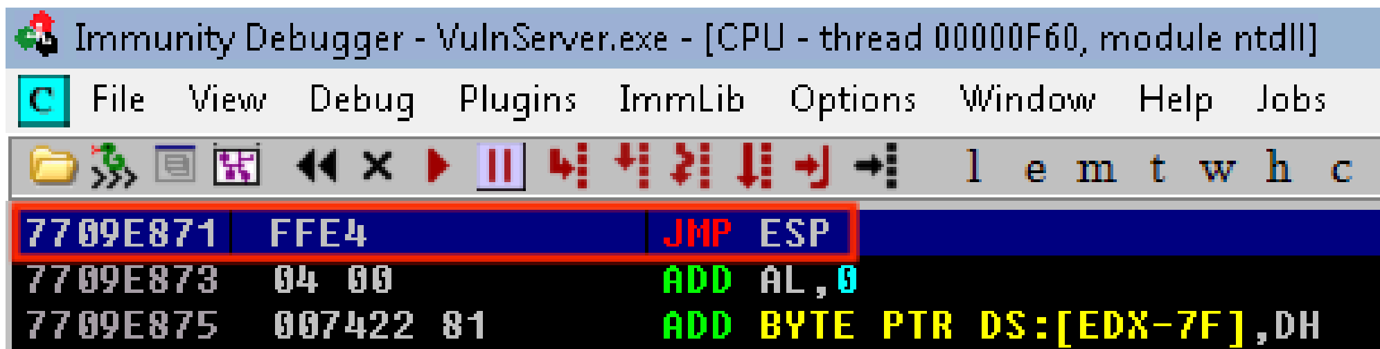
Figure 103: Impermanent JMP ESP instruction located at 7709E871, pre-restart
