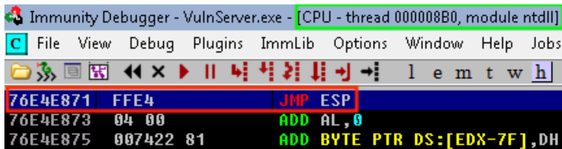
Figure 29: Found JMP ESP instruction in the paused thread post restart
