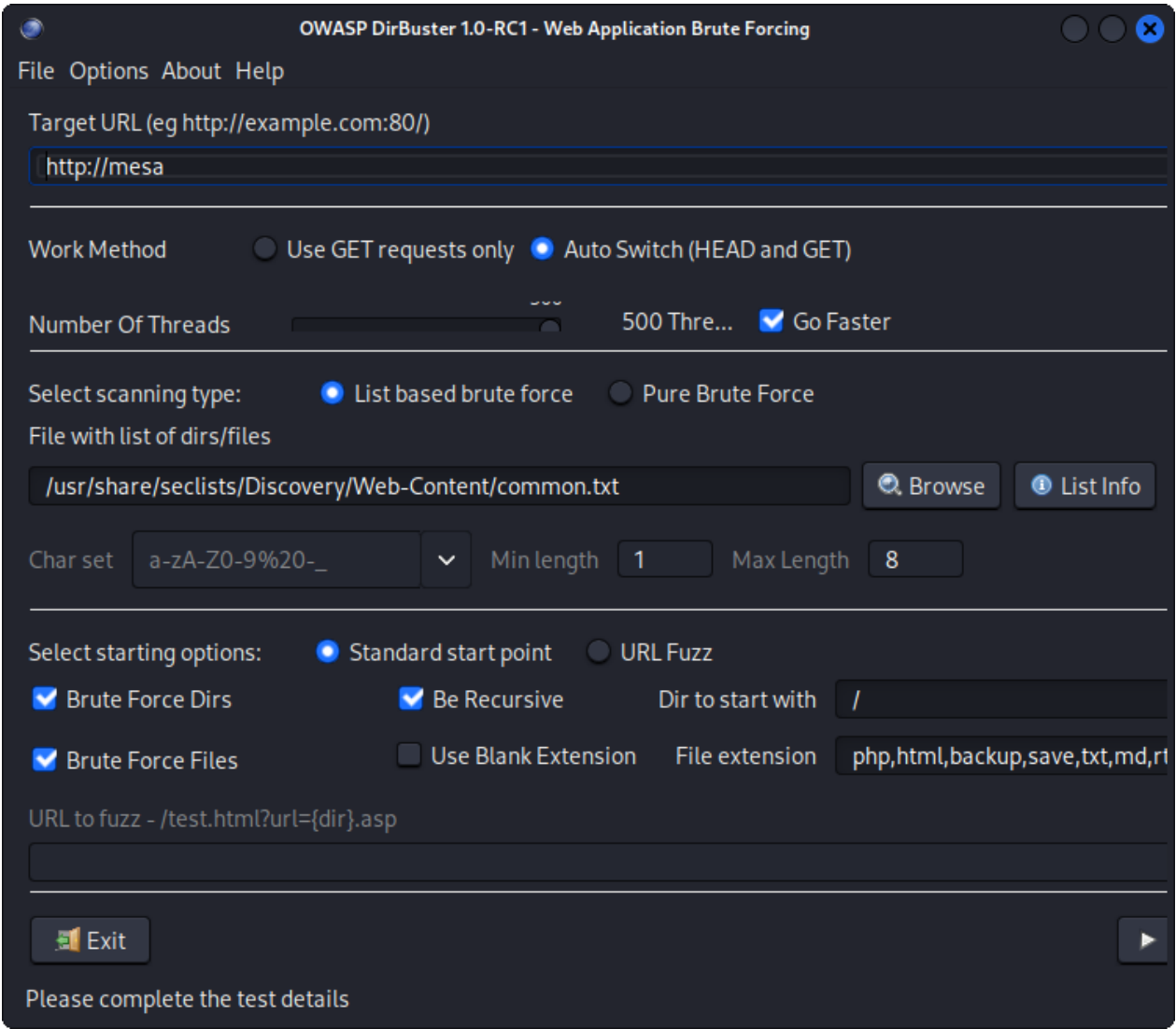
Figure 49: Dirbuster setup
