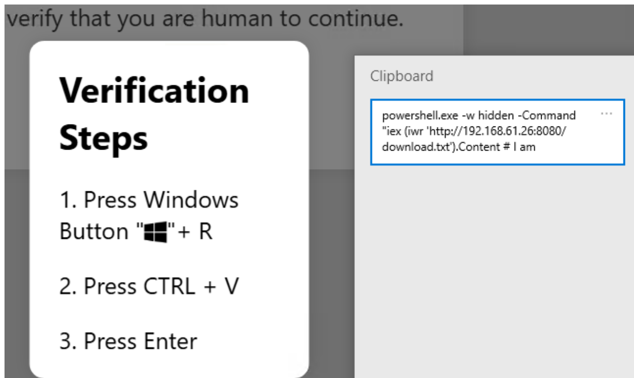
Figure 140: Popup instructing user to execute PowerShell command stored in clipboard
