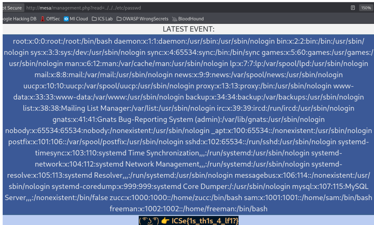
Figure 86: File inclusion of /etc/passwd
