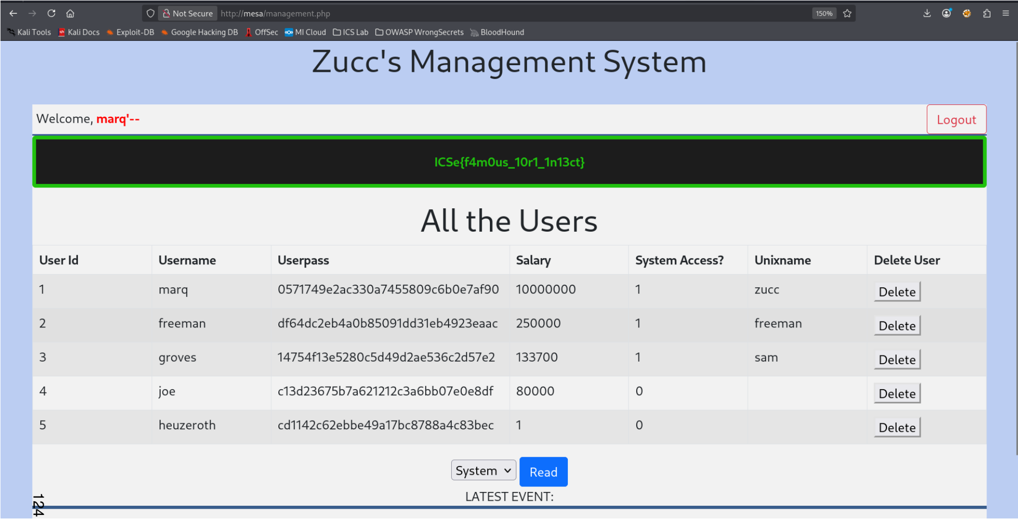
Figure 146: Successful SQL injection attempt 2
