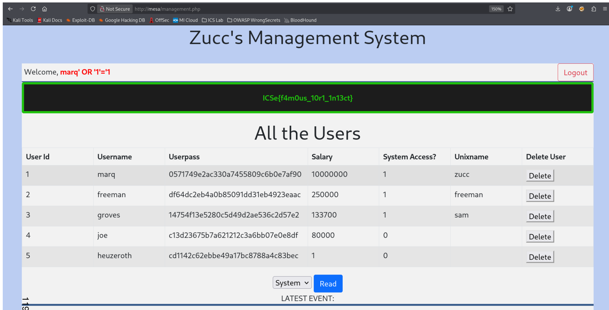
Figure 158: Successful SQL injection attempt 3 - Jump to reference
