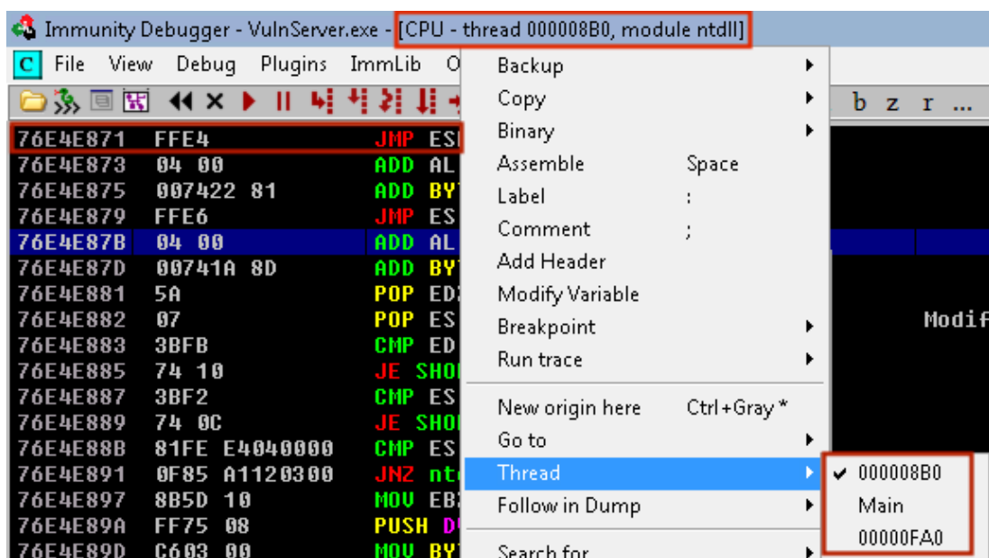
Figure 30: JMP ESP command not located in main thread
