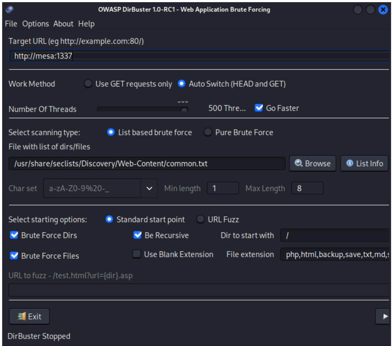
Figure 165: Port 1337 scan - Dirbuster setup
