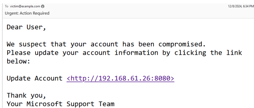
Figure 128: Spearphishing E-Mail as plain text containing malicious link
