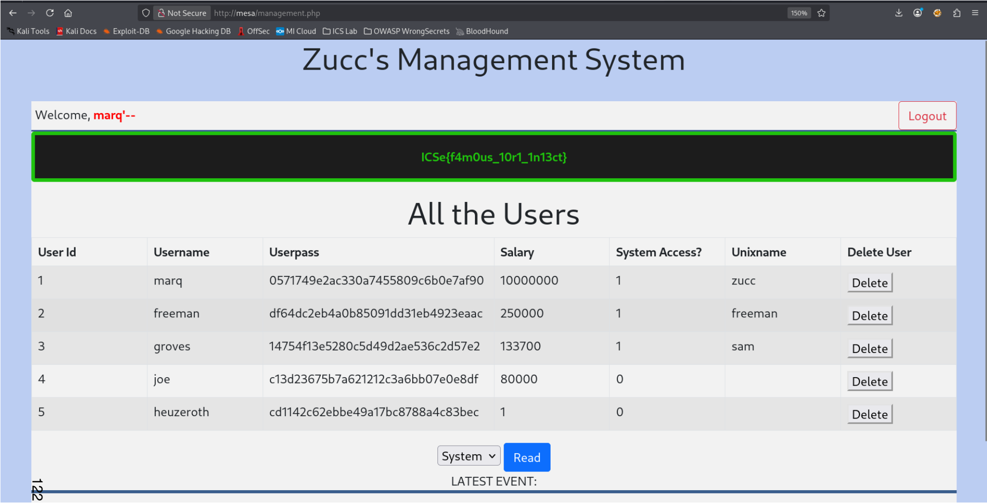
Figure 159: Successful SQL injection attempt 2
