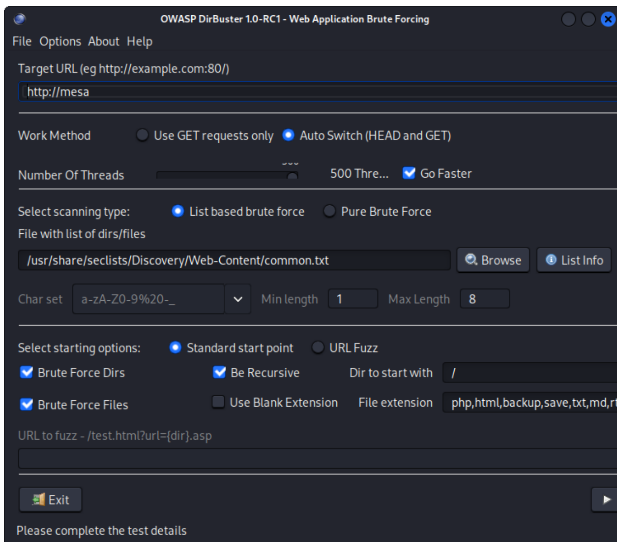
Figure 49: Dirbuster setup
