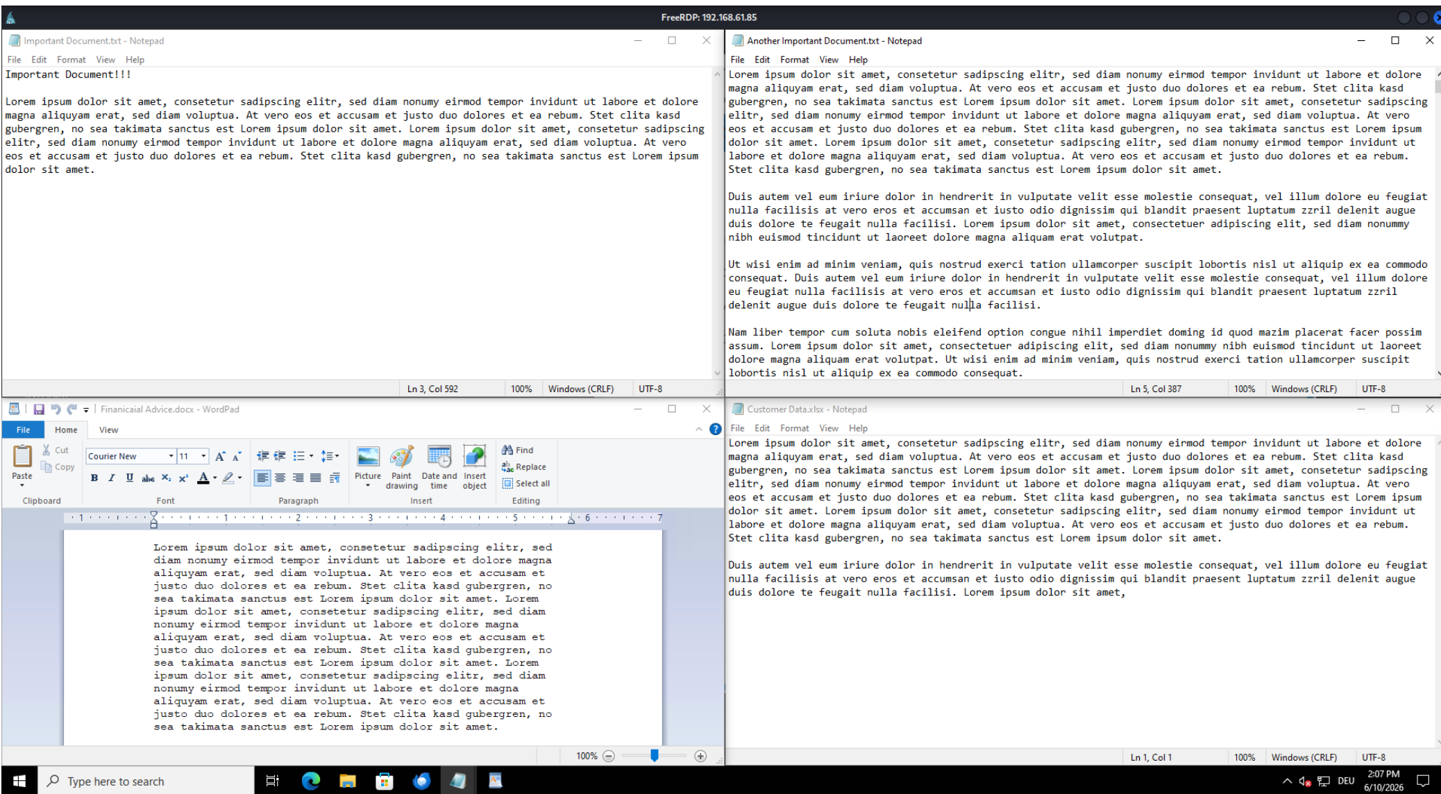
Figure 176: Decrypted files
