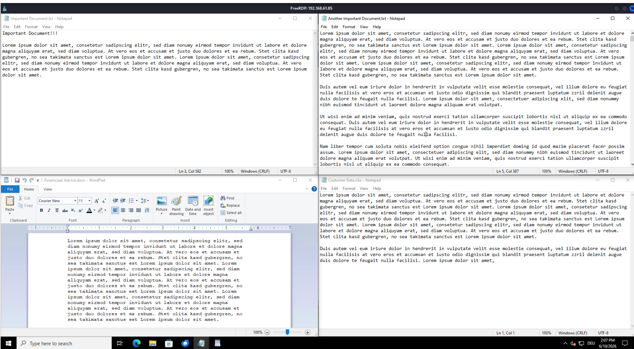
Figure 179: Decrypted files
