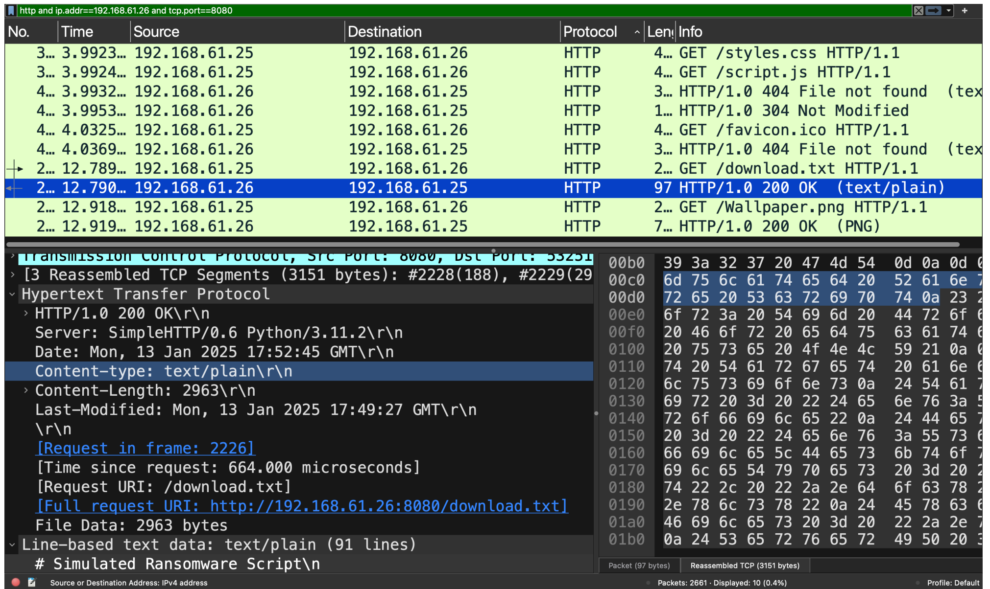
Figure 138: Wireshark trace after filtering
