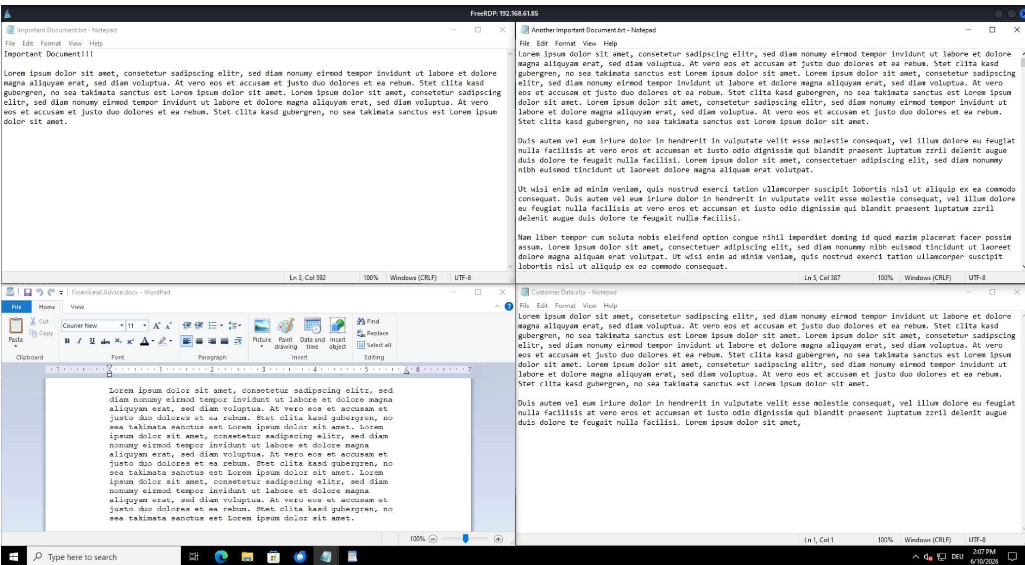
Figure 180: Decrypted files
