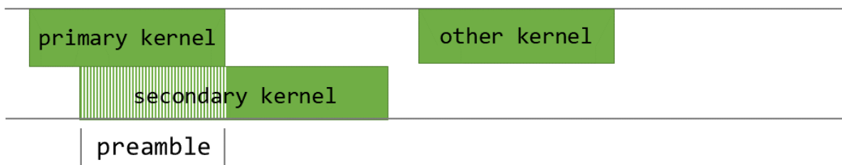
Figure 44: Concurrent execution of primary_kernel and secondary_kernel
