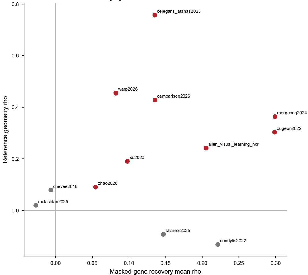
Fig2 global AtlasLift reference atlas
