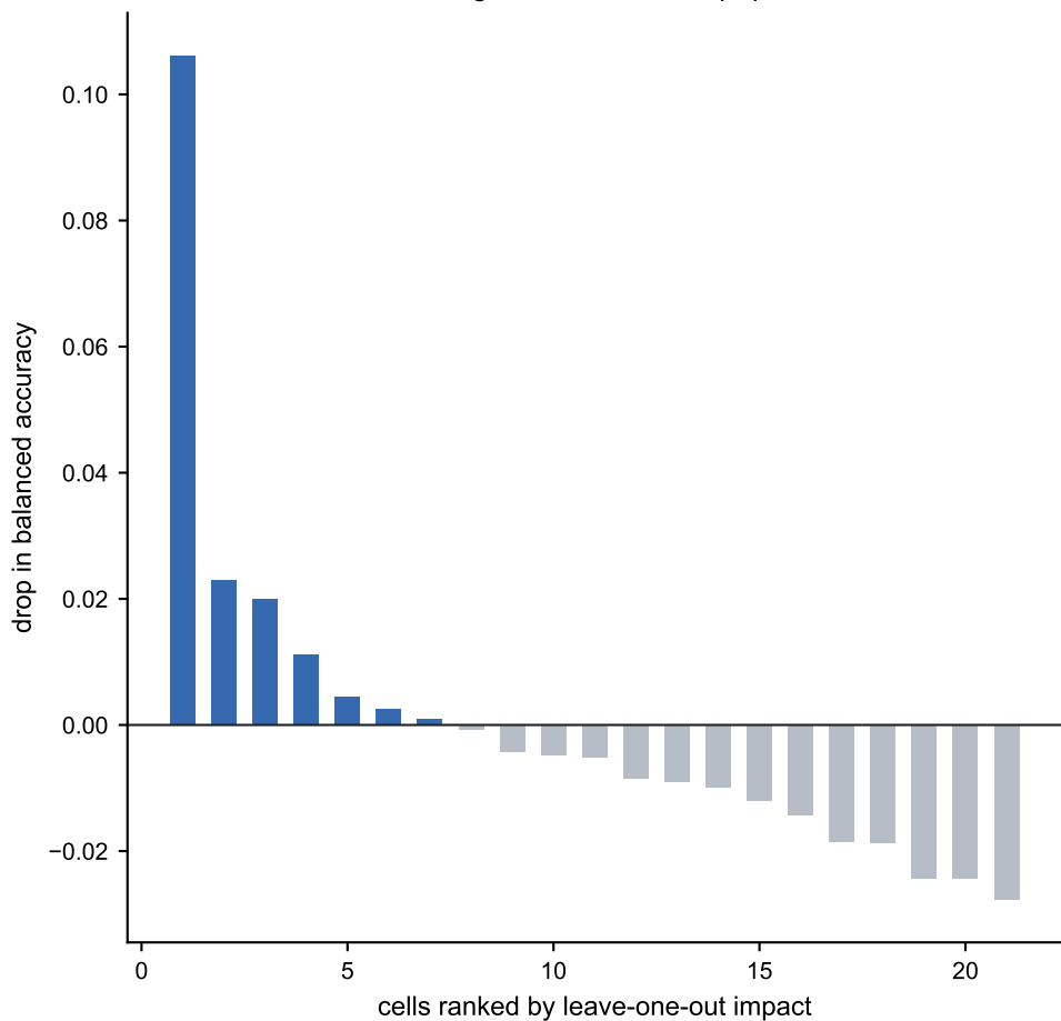
ANM181: no single cell carries the population code
