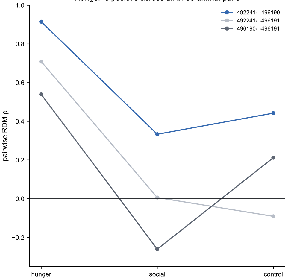
Hunger is positive across all three animal pairs
