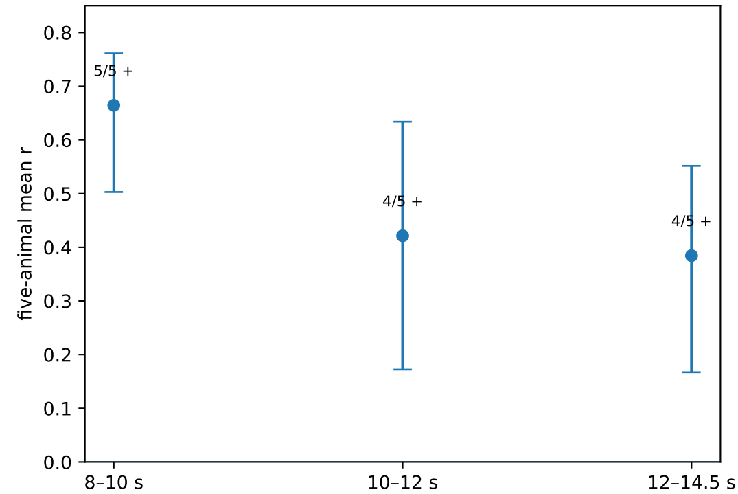
D Animal-level delayed-window meta-analysis
