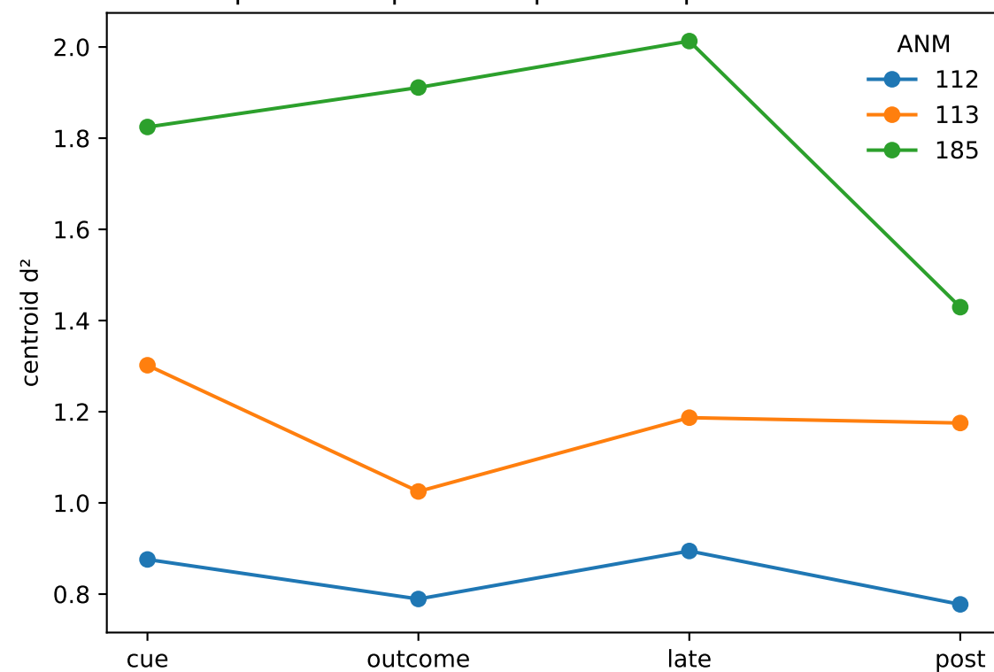
D Population separation spans multiple event windows
