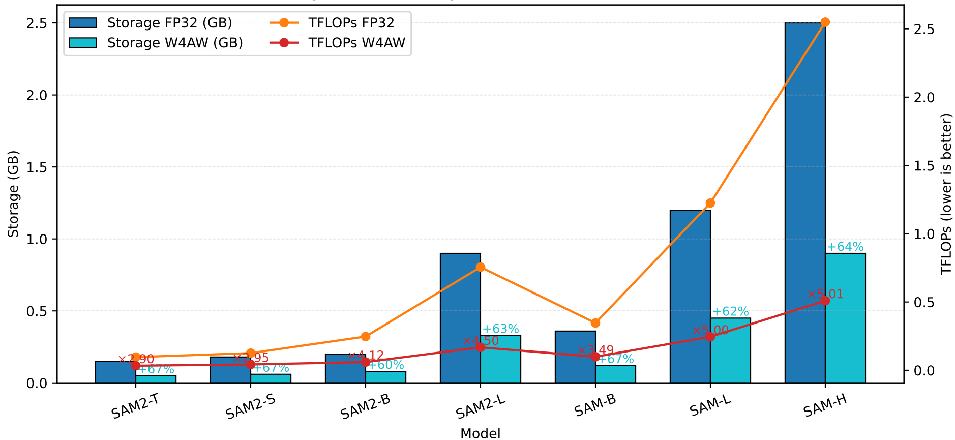
Storage (GB) and Compute (TFLOPs): FP32 vs W4AW
