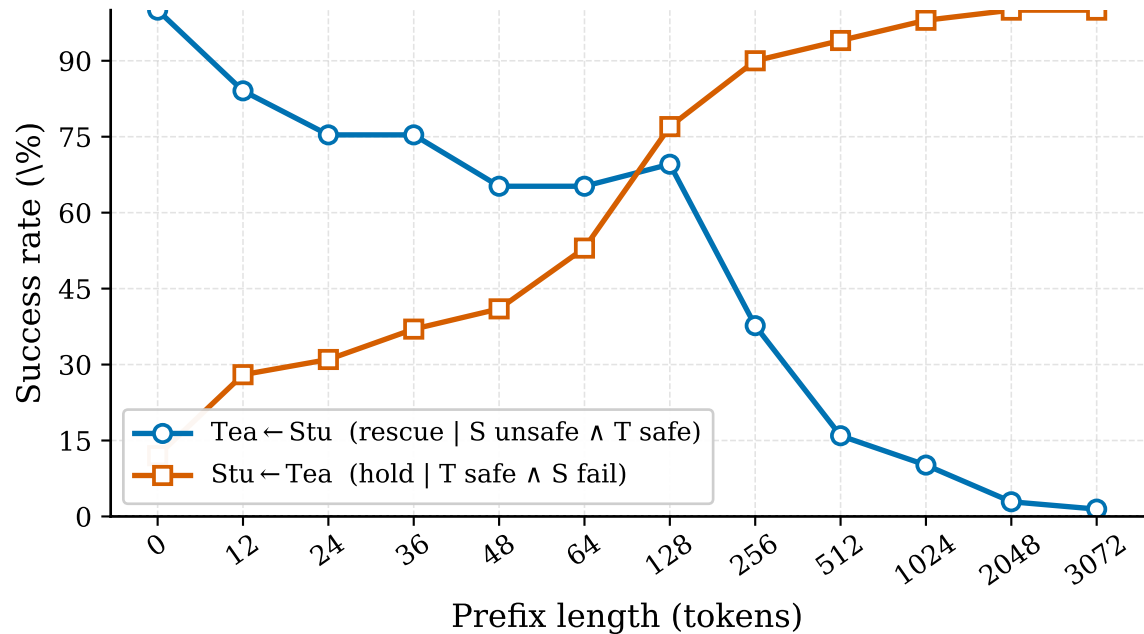
R1-Distill-1.5B
