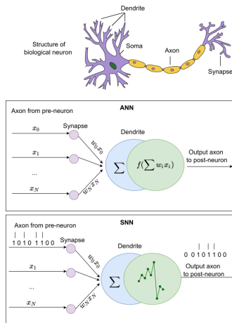
Biological neuron vs Artificial Neural Network (ANN) vs Spiking Neural Network (SNN) (as in [snn])
