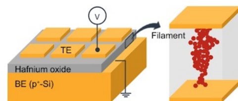
Memristors
