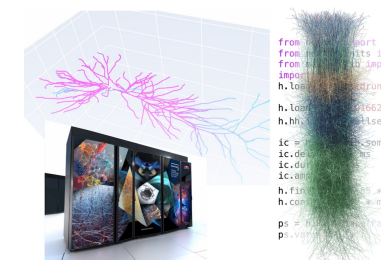
NEURON
