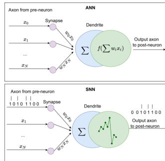
Biological neuron vs Artificial Neural Network (ANN) vs Spiking Neural Network (SNN) (as in [2])
