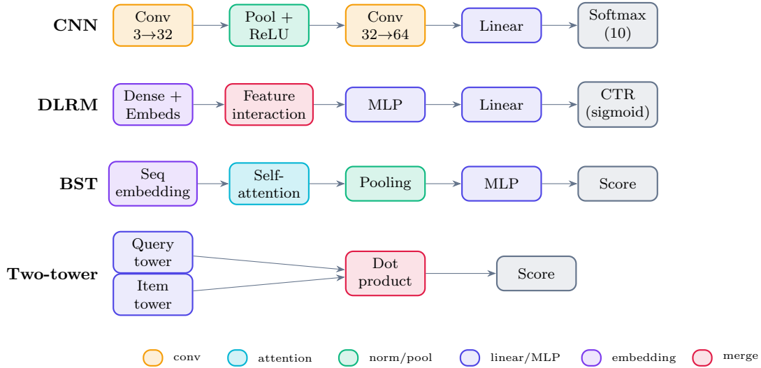
Figure 6: Four of the twelve curated tasks, as typed graphs, coloured by layer type (the same convention the Neurarch canvas uses): a CIFAR-10 CNN, a DLRM click-through-rate ranker, a Behavior Sequence Transformer (which requires an attention layer), and a two-tower retrieval model (two encoders scored by a dot product). These are the states an agent edits and the verifier grades.
