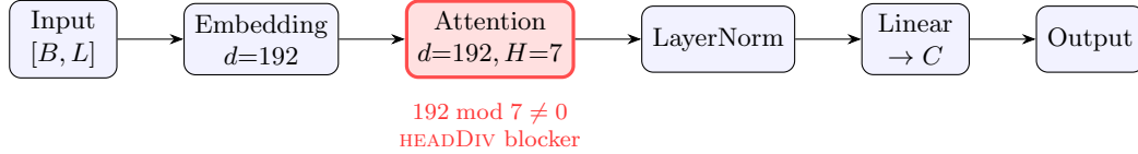
Figure 2: A task state as a typed graph, and a hard blocker the verifier returns in O(1) at the attention node: \text{embedDim}=192 is not divisible by \text{numHeads}=7 (Algorithm 1, line 4). Because widths and divisibility are typed-node properties, this check is a pure function; on free-form code it would require executing the model. The input carries shape [B, L] ( B batch, L sequence length), widening to [B, L, 192] after the embedding. The repair task asks the policy to fix exactly this in \leq 2 edits without rebuilding.
