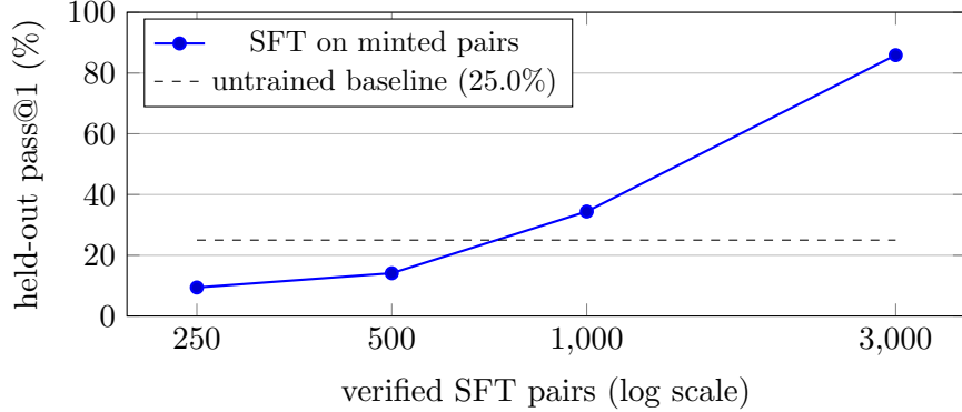
Figure 5: Held-out pass@1 vs. number of environment-minted verified SFT pairs (Qwen2.5-1.5B, LoRA, 2 epochs, seed-999 split, n=64 ). The curve is steep: below \sim 1k pairs the half-learned format underperforms the raw instruct model; 3k pairs reach 85.9%. Pairs are free to mint, so the x-axis costs seconds of generation.
