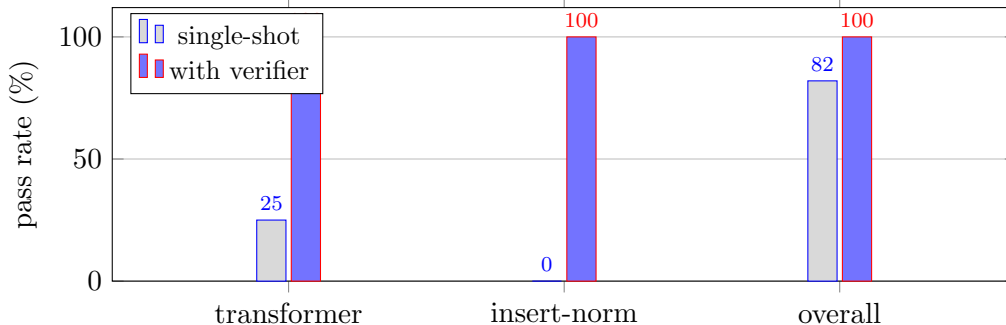
Figure 4: Verifier-in-the-loop lift for claude-sonnet-4-6 . The overall gain (82 \rightarrow 100) lands entirely on the two families a frontier model finds hard; the eight saturated families (all at 100%) are omitted for clarity.
