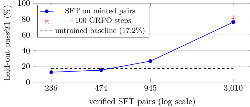
Figure 6: Held-out pass@1 vs. environment-minted verified SFT pairs (Qwen2.5-1.5B, LoRA, 2 epochs; corrected zero-overlap protocol, seed-999 split, n=192 ). The x-axis is the number of verified rows actually trained on (nominal mints of 250/500/1000/3000 minus rows colliding with the holdout). The curve is steep and non-monotonic: below \sim 1k pairs the half-learned edit format underperforms the untrained model (17.2%, dashed); 945 pairs cross above (26.6%); 3,010 reach 76.0%. Pairs are free to mint, so the x-axis costs seconds of generation. The star marks 100 GRPO steps on the 3k checkpoint (80.2%).
