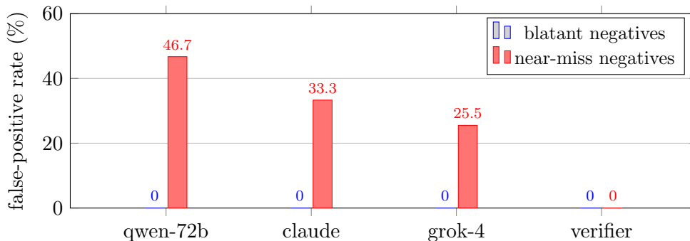
Figure 7: The collapse, visually: LLM reward models that never approve a blatantly broken design approve 26–47% of near-miss designs one edit from correct. The deterministic verifier is 0% on both tiers by construction.
