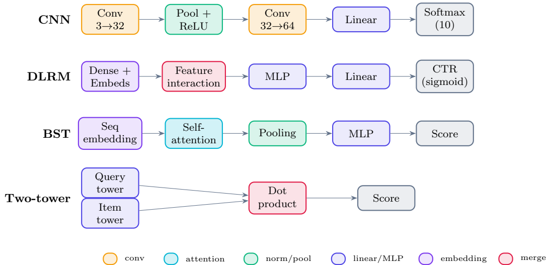
Figure 8: Four of the twelve curated tasks, as typed graphs, coloured by layer type (the same convention the Neurarch canvas uses): a CIFAR-10 CNN, a DLRM click-through-rate ranker, a Behavior Sequence Transformer (which requires an attention layer), and a two-tower retrieval model (two encoders scored by a dot product). These are the states an agent edits and the verifier grades.
