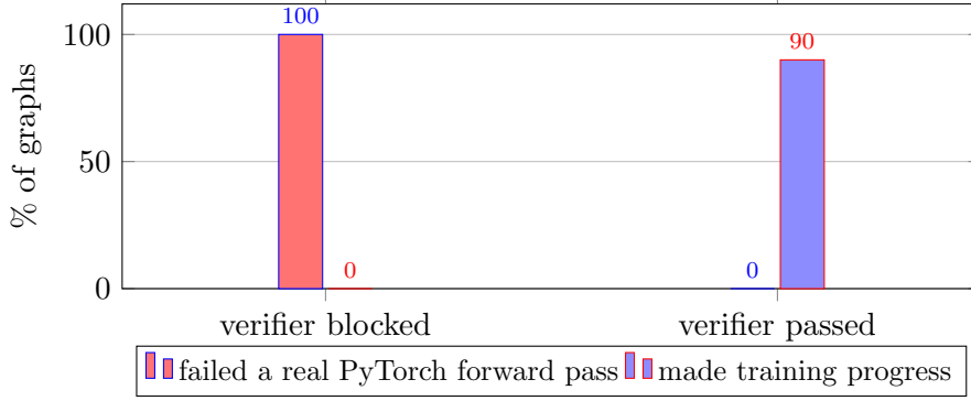
Figure 3: Grounding study (264 graphs, two seeds: 80 clean, 96 blocked, 88 width-corrupted). Every graph the verifier blocked (96/96) failed a real PyTorch forward pass; every clean graph passed and constructed (80/80), with 90% making training progress. The width-corrupted class (not shown) passes the transparent rubric yet fails 88/88 forward passes – the rubric’s blind spot, measured in the text.
