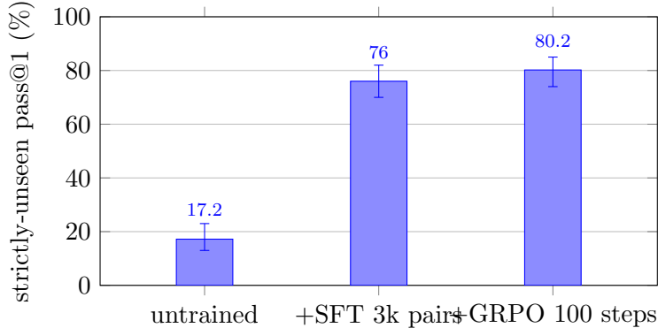
Figure 5: The corrected-protocol checkpoint chain (Qwen2.5-1.5B, seed-999 strictly-unseen split, n=192 ; error bars are Wilson 95% intervals). SFT on 3k environment-minted verified pairs lifts pass@1 from 17.2% to 76.0% with non-overlapping intervals; 100 GRPO steps on the merged SFT checkpoint reach 80.2%, a level an independent GRPO rerun reproduces exactly.
