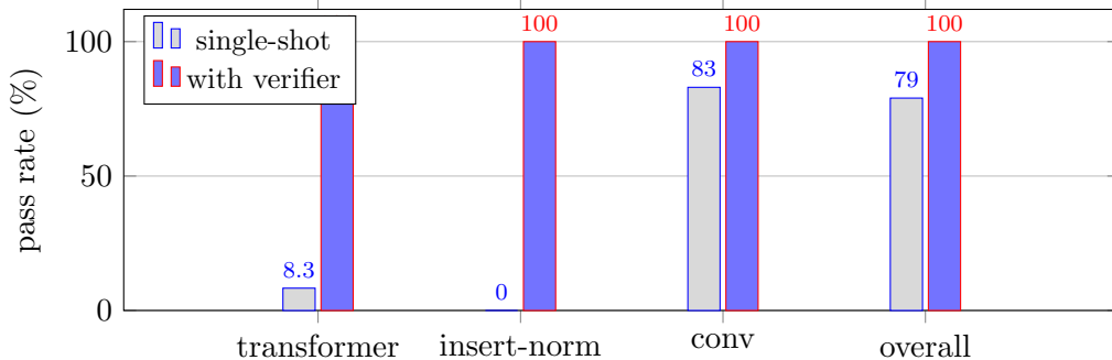
Figure 4: Verifier-in-the-loop lift for claude-sonnet-4-6 . The overall gain (79 \rightarrow 100; 25 tasks rescued) is concentrated on the two families the model finds hard (11 fixes on the transformer encoder, 12 on insert-norm), with the convolutional classifier contributing the remaining 2; the seven families already at 100% single-shot are omitted.
