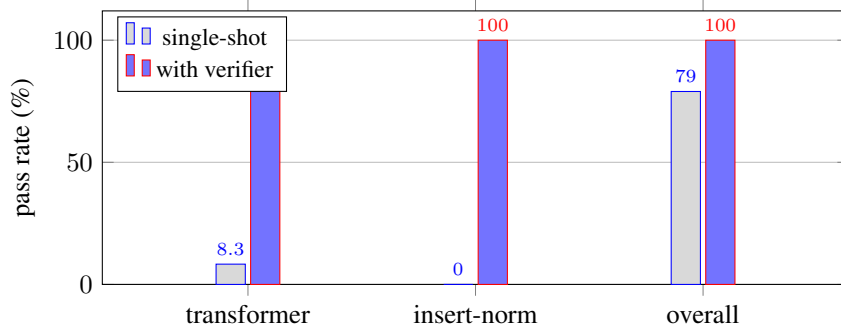
Figure 4: Verifier-in-the-loop lift for claude-sonnet-4-6 . The overall gain (79 → 100) lands entirely on the two families a frontier model finds hard; the eight saturated families (all at 100%) are omitted for clarity.
