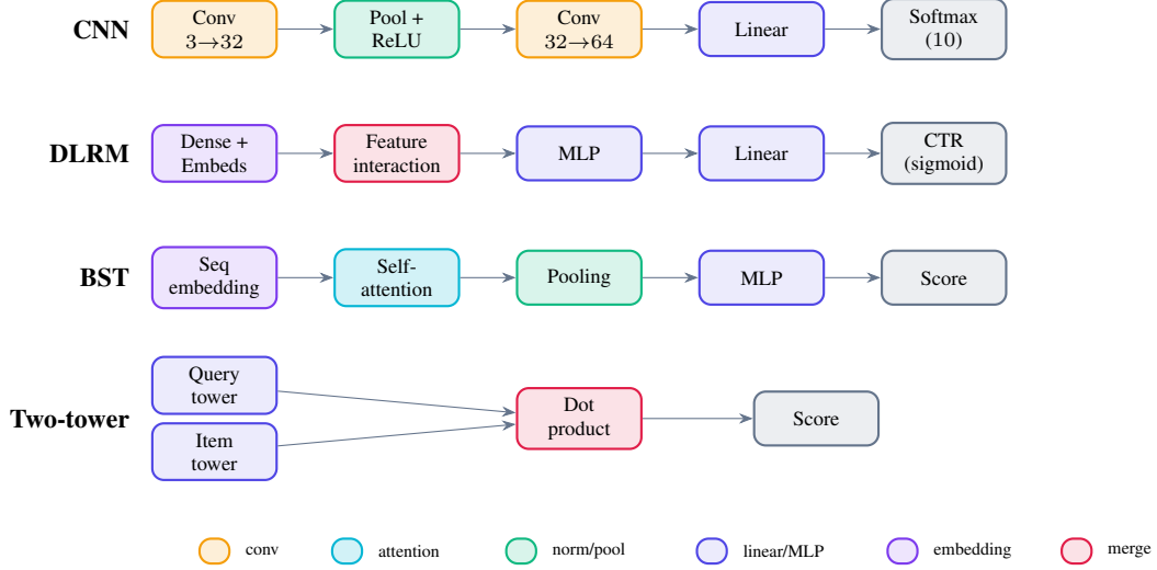
Figure 8: Four of the twelve curated tasks, as typed graphs, coloured by layer type (the same convention the Neurarch canvas uses): a CIFAR-10 CNN, a DLRM click-through-rate ranker, a Behavior Sequence Transformer (which requires an attention layer), and a two-tower retrieval model (two encoders scored by a dot product). These are the states an agent edits and the verifier grades.
