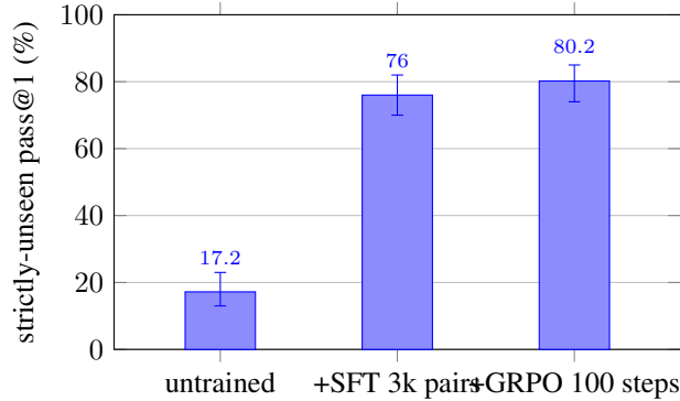
Figure 5: The corrected-protocol checkpoint chain (Qwen2.5-1.5B, seed-999 strictly-unseen split, n=192 ; error bars are Wilson 95% intervals). SFT on 3k environment-minted verified pairs lifts pass@1 from 17.2% to 76.0% with non-overlapping intervals; 100 GRPO steps on the merged SFT checkpoint reach 80.2%, a level an independent GRPO rerun reproduces exactly.
