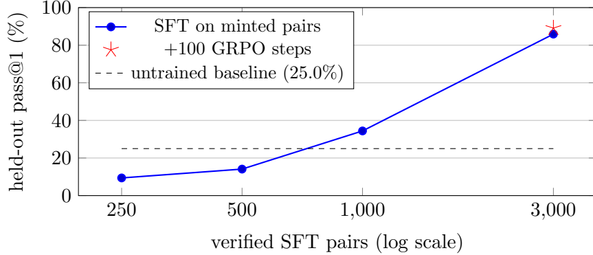
Figure 6: Held-out pass@1 vs. number of environment-minted verified SFT pairs (Qwen2.5-1.5B, LoRA, 2 epochs, seed-999 split, n=64 ). The curve is steep: below \sim 1k pairs the half-learned format underperforms the raw instruct model; 3k pairs reach 85.9%. Pairs are free to mint, so the x-axis costs seconds of generation. The star marks 100 GRPO steps on the 3k checkpoint. Curve measured under the pre-audit v1 protocol (includes seen tasks); the corrected zero-overlap 3k numbers are 76.0% (SFT) and 80.2% (+GRPO) at n=192 .
