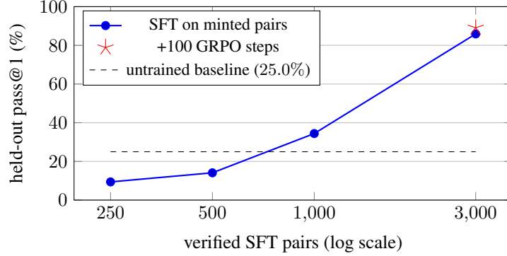
Figure 5: Held-out pass@1 vs. number of environment-minted verified SFT pairs (Qwen2.5-1.5B, LoRA, 2 epochs, seed-999 split, n=64 ). The curve is steep: below \sim 1 k pairs the half-learned format underperforms the raw instruct model; 3k pairs reach 85.9%. Pairs are free to mint, so the x-axis costs seconds of generation. The star marks 100 GRPO steps on the 3k checkpoint. Curve measured under the pre-audit v1 protocol (includes seen tasks); the corrected zero-overlap 3k numbers are 68.8% (SFT) and 71.9% (+GRPO).
