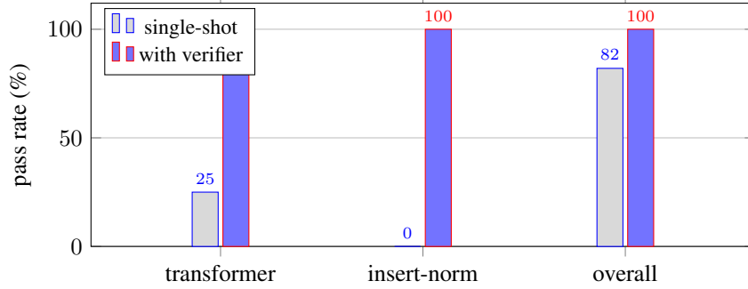
Figure 4: Verifier-in-the-loop lift for claude-sonnet-4-6. The overall gain (82 \rightarrow 100) lands entirely on the two families a frontier model finds hard; the eight saturated families (all at 100%) are omitted for clarity.
