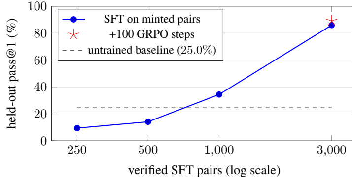
Figure 5: Held-out pass@1 vs. number of environment-minted verified SFT pairs (Qwen2.5-1.5B, LoRA, 2 epochs, seed-999 split, n=64 ). The curve is steep: below \sim 1k pairs the half-learned format underperforms the raw instruct model; 3k pairs reach 85.9%. Pairs are free to mint, so the x-axis costs seconds of generation. The star marks 100 GRPO steps on the 3k checkpoint. Curve measured under the pre-audit v1 protocol (includes seen tasks); the corrected zero-overlap 3k numbers are 68.8% (SFT) and 71.9% (+GRPO).
